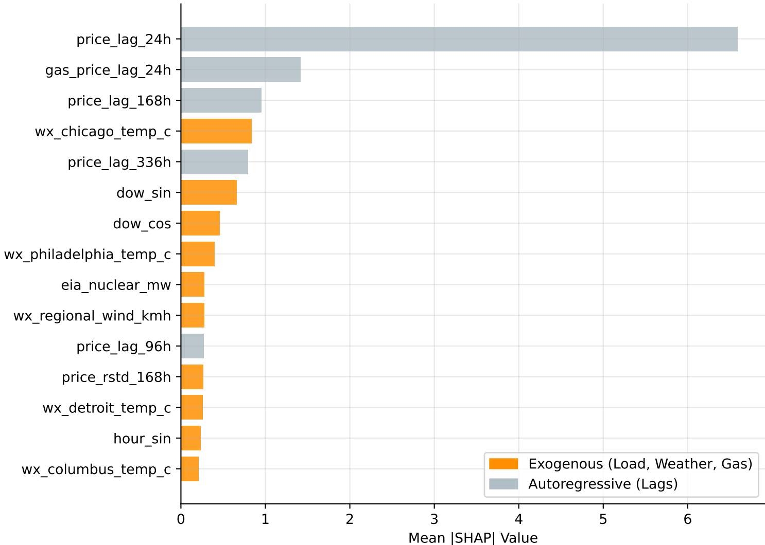
SHAP Feature Importance (LightGBM, PJM)
