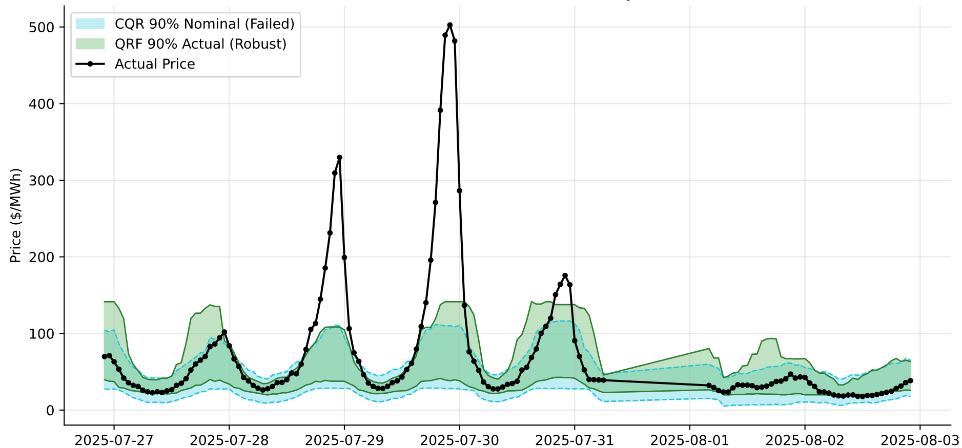
CQR vs. QRF Prediction Intervals (PJM)
