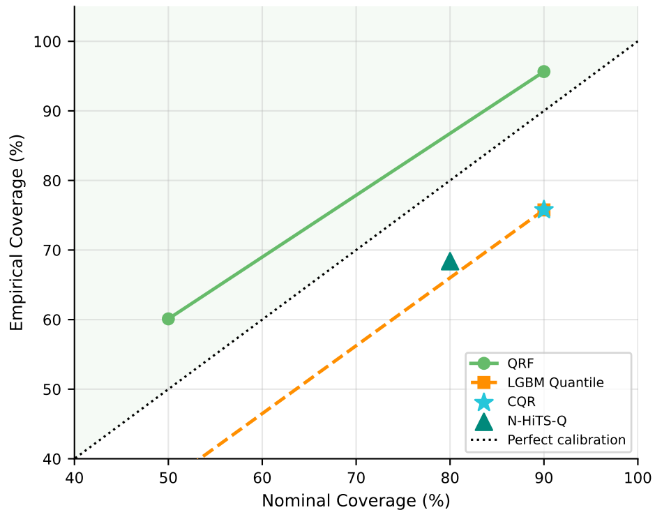
ERCOT — Reliability Diagram
