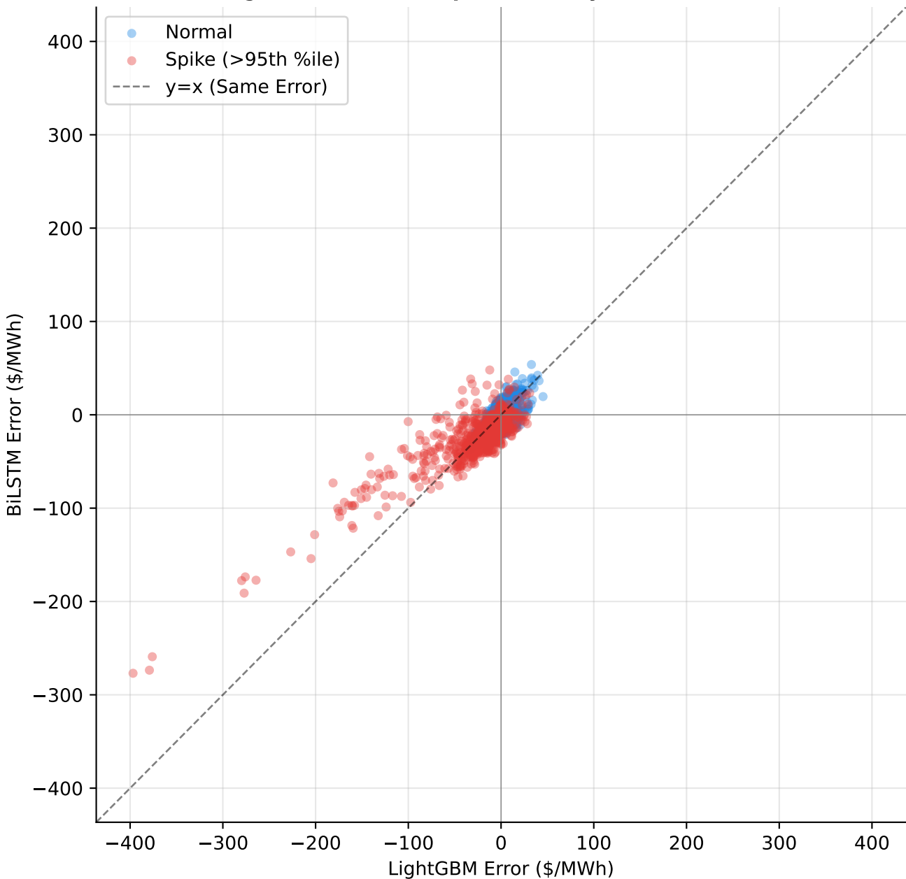
Figure D: Error Complementarity (Trees vs RNN)
