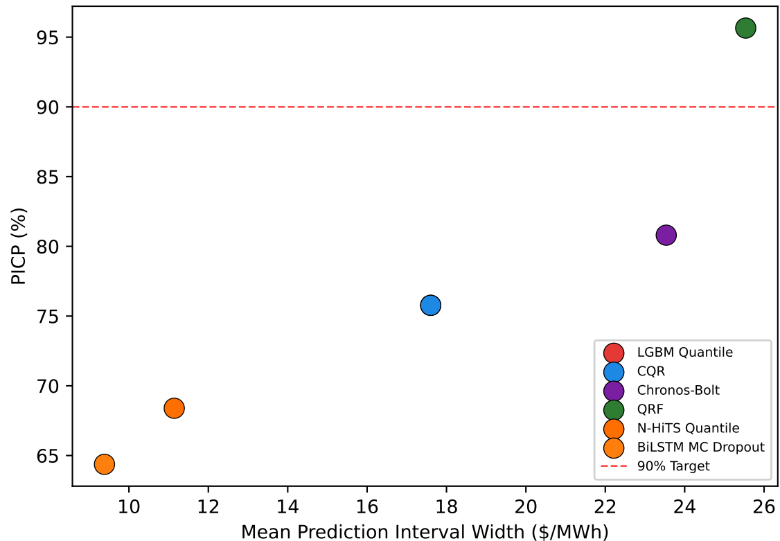
ERCOT: Coverage vs Sharpness
