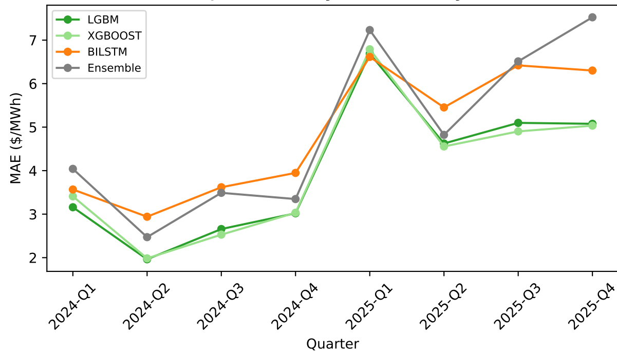
PJM: Quarterly MAE Stability
