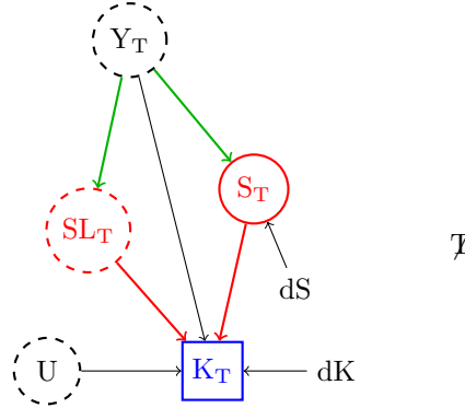
Figure 4: DAG of causalities with hierarchical modeling with stratified by T (Model 2) - See Figure 1 for notations.
