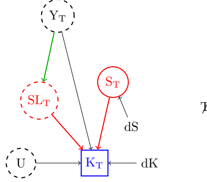
Figure 5: DAG of causalities with some hierarchical modeling with stratified by T (Model 3) - causality of Y -> S are ignored as it is represented in auto-correlation between S and SL, though Y -> SL is needed to estimate hidden SL. See Figure 1 for notations.
