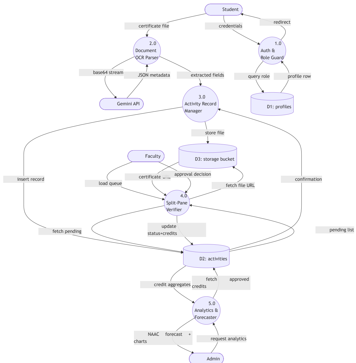
Fig. 4.6(b): DFD Level 1 — Internal Processes
