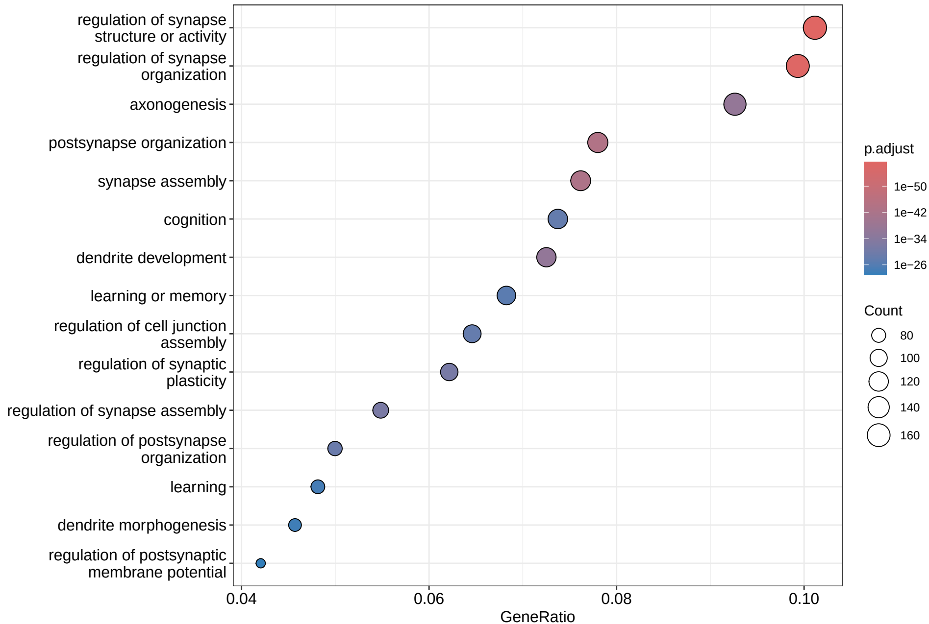
NEIL2KO_3h_ipsilateral_vs_contralateral Down GO_BP
