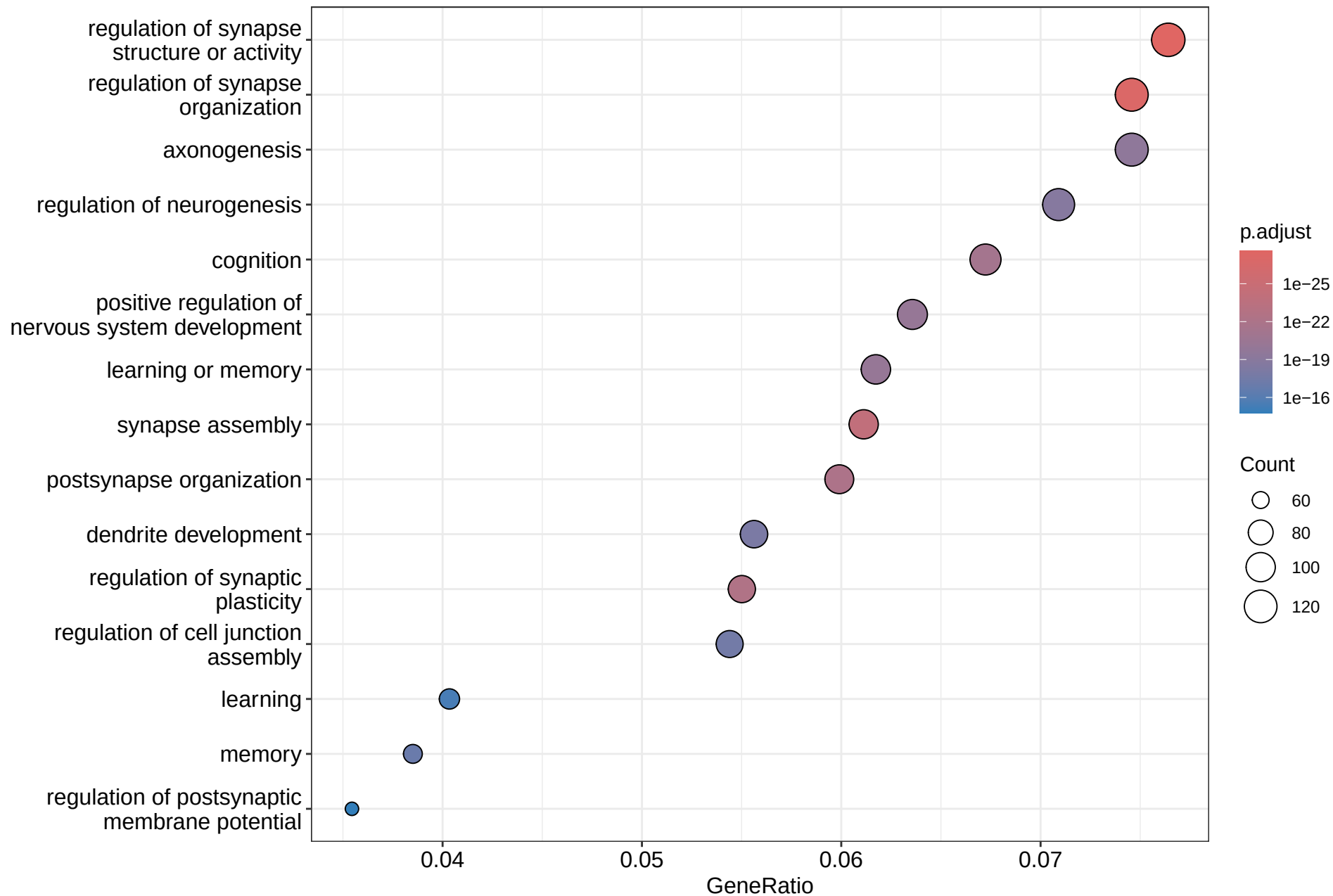
WT_3h_ipsilateral_vs_contralateral All GO_BP
