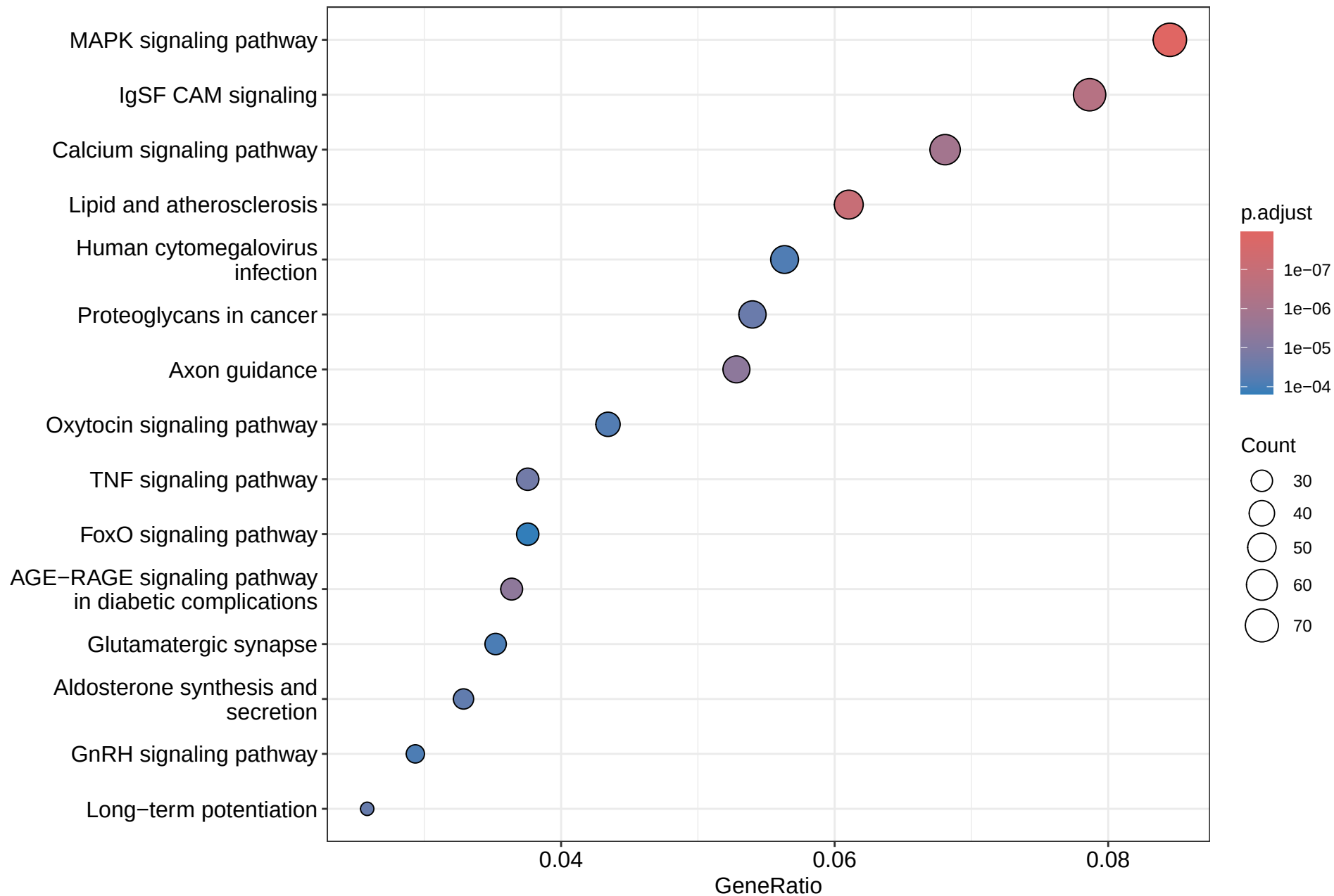
WT_3h_ipsilateral_vs_contralateral All KEGG
