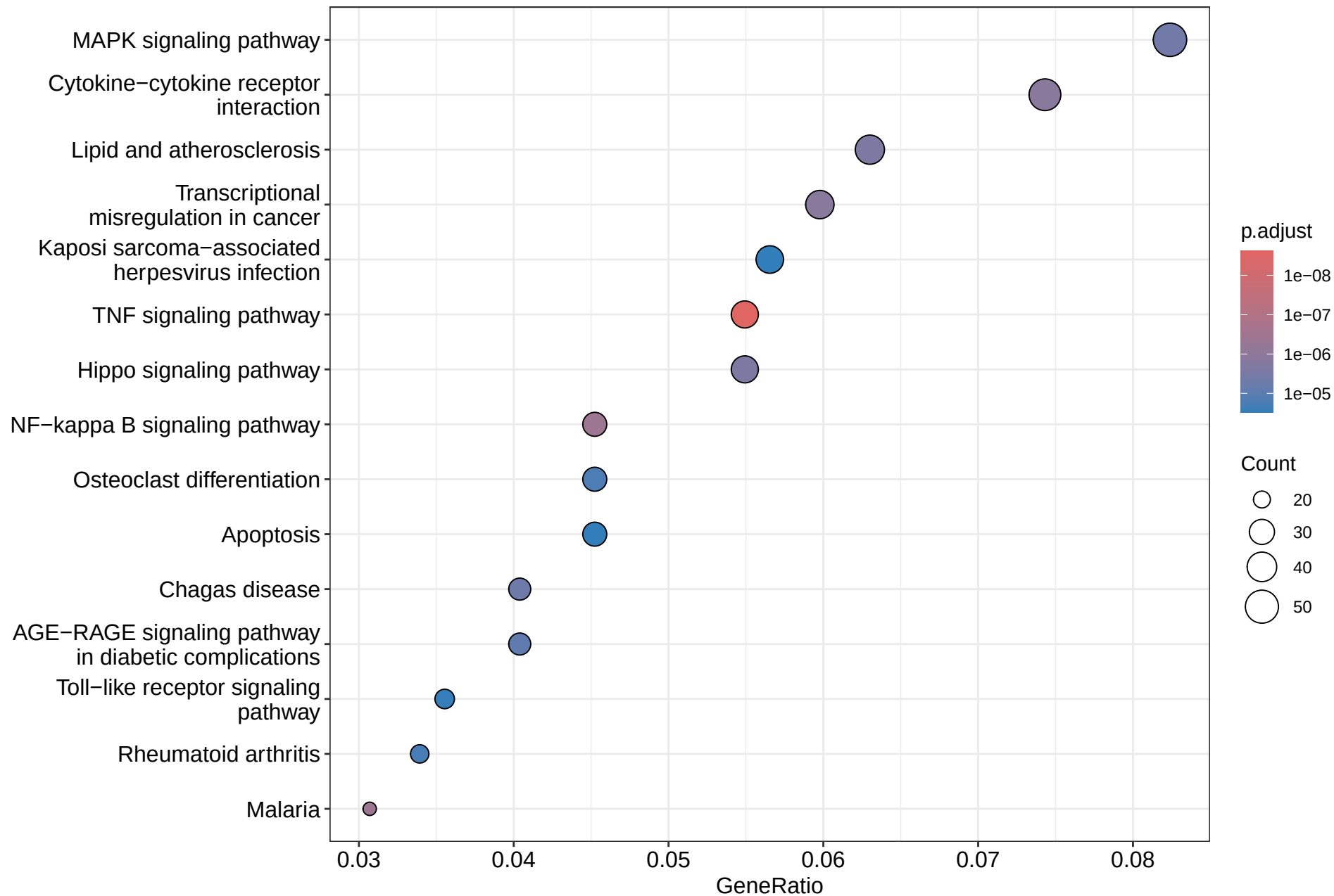
WT_6h_ipsilateral_vs_contralateral Up KEGG
