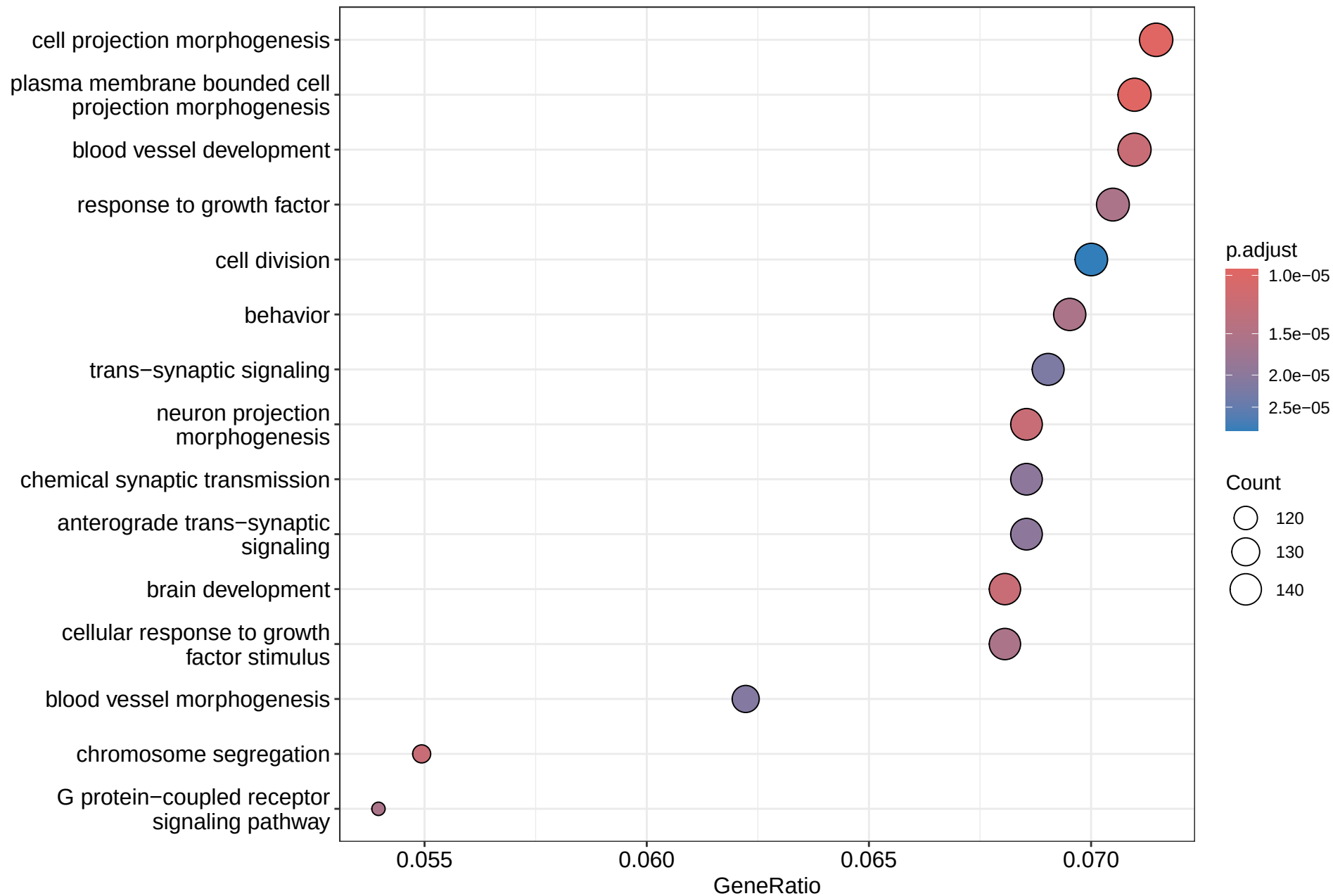
Microglia_1d_HI_vs_Control Down GO_BP
