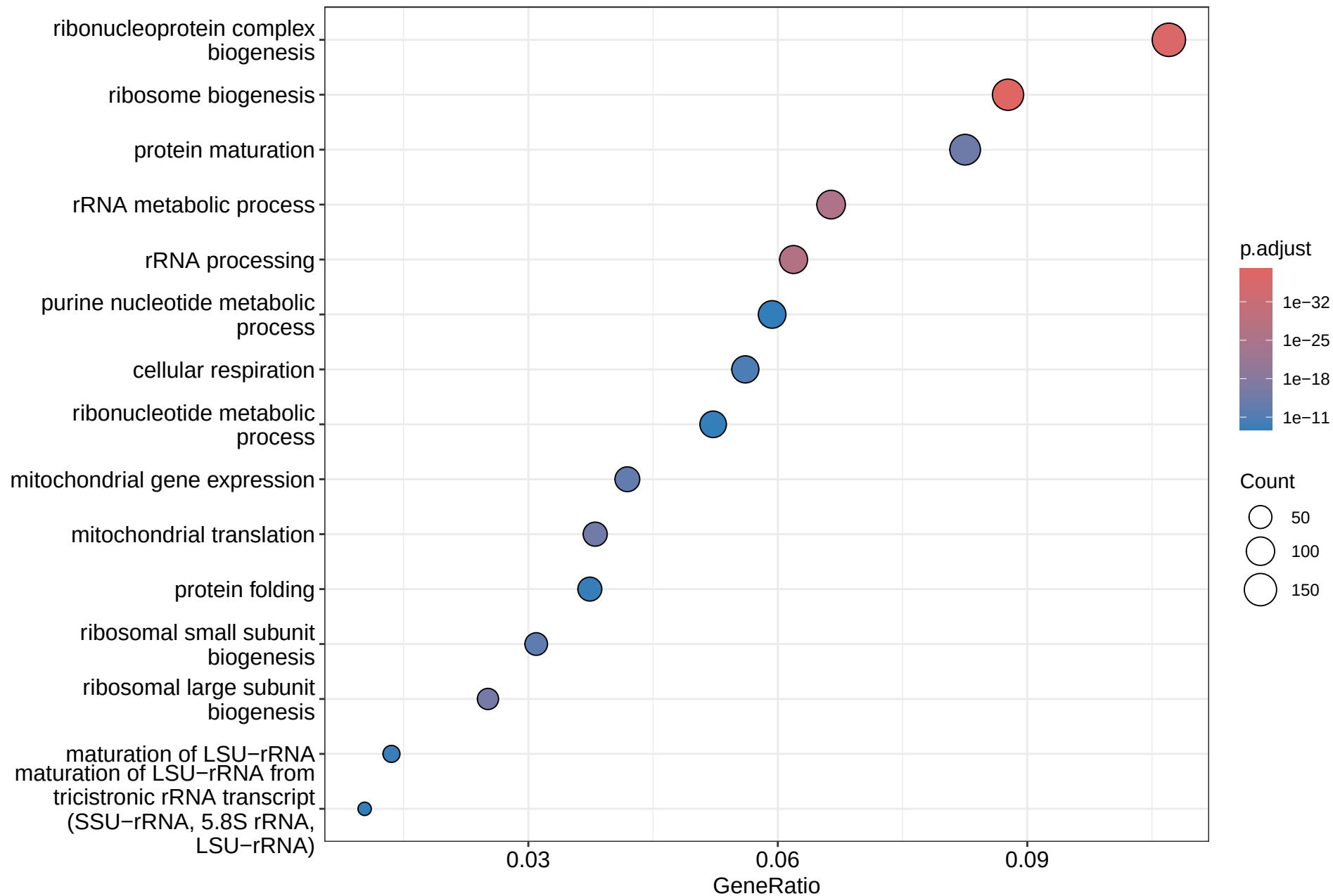
Microglia_1d_HI_vs_Control Up GO_BP
