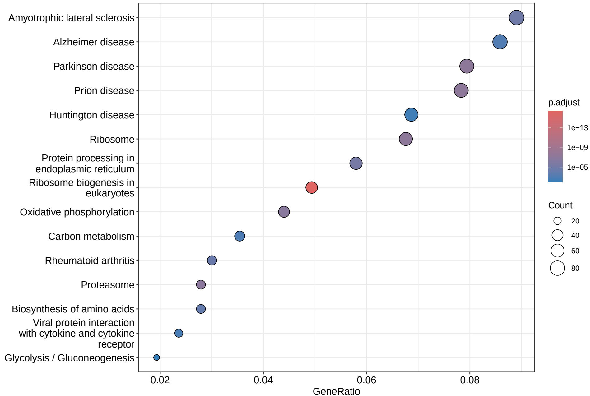
Microglia_1d_HI_vs_Control Up KEGG
