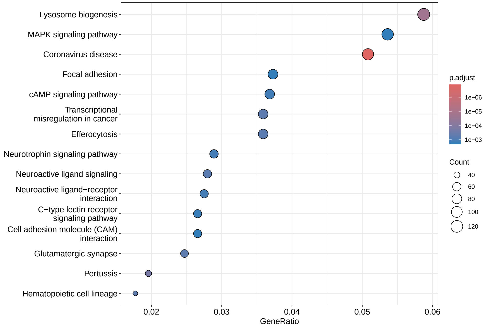
Microglia_3d_HI_vs_Control All KEGG
