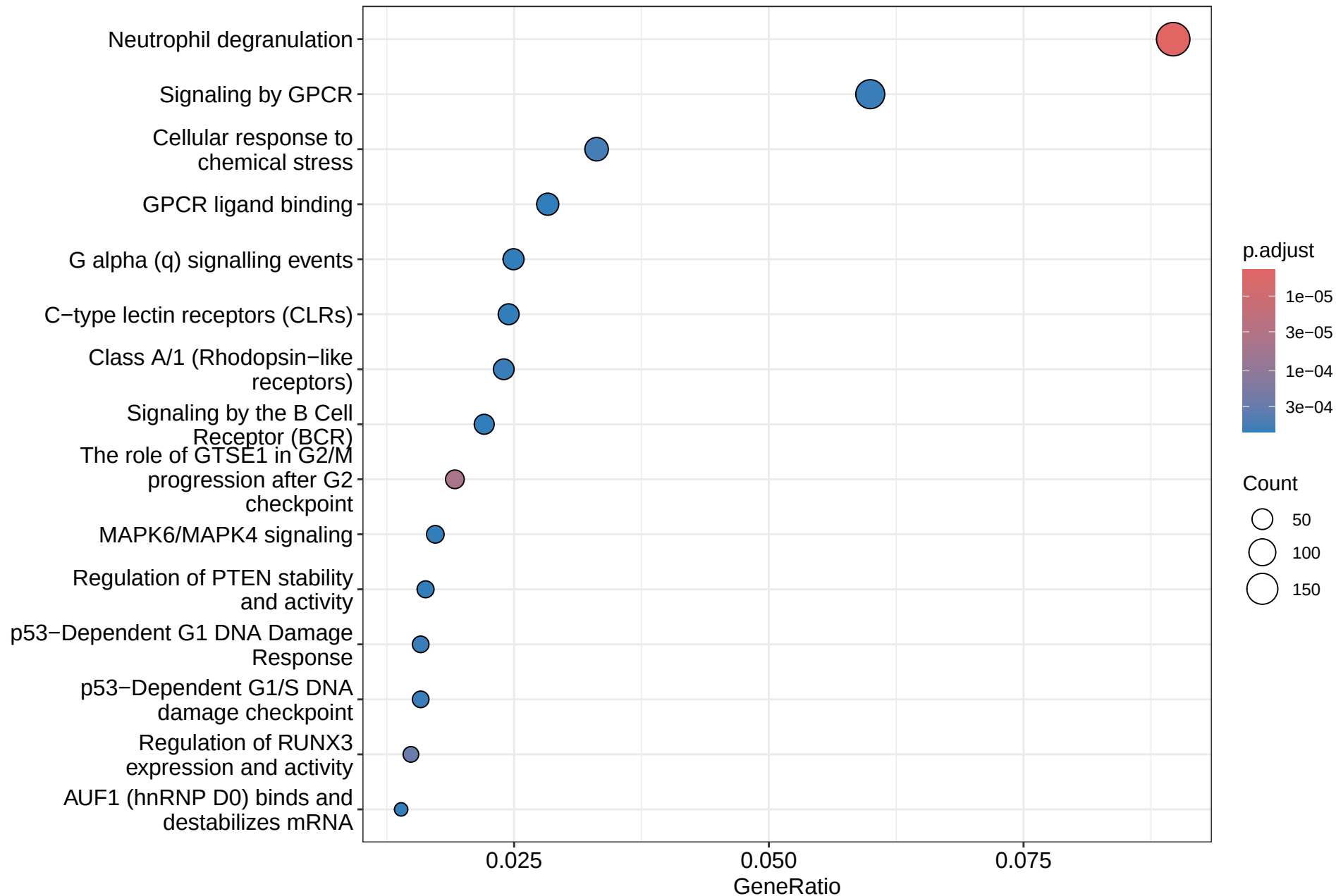
Microglia_1d_HI_vs_Control All Reactome
