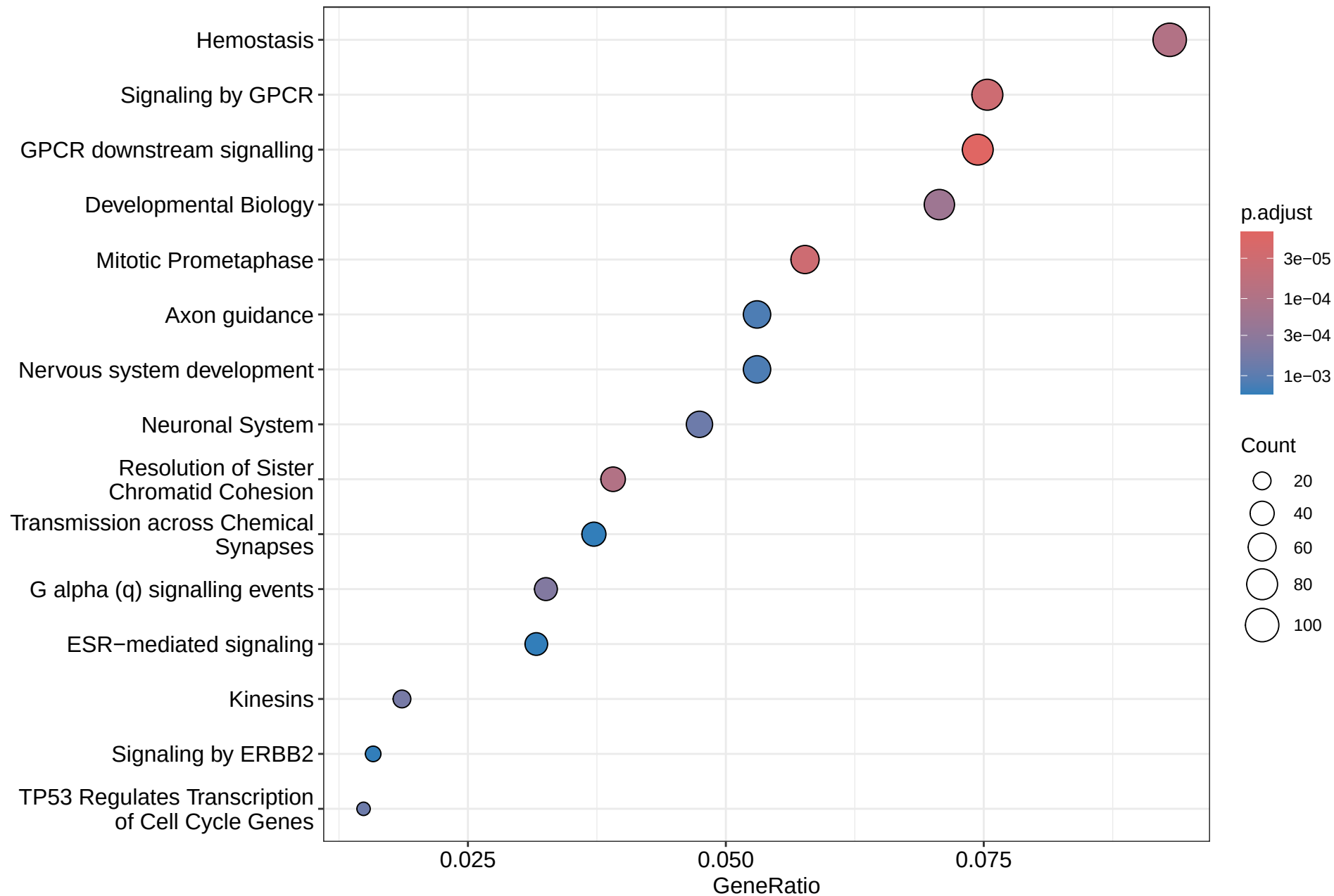
Microglia_1d_HI_vs_Control Down Reactome
