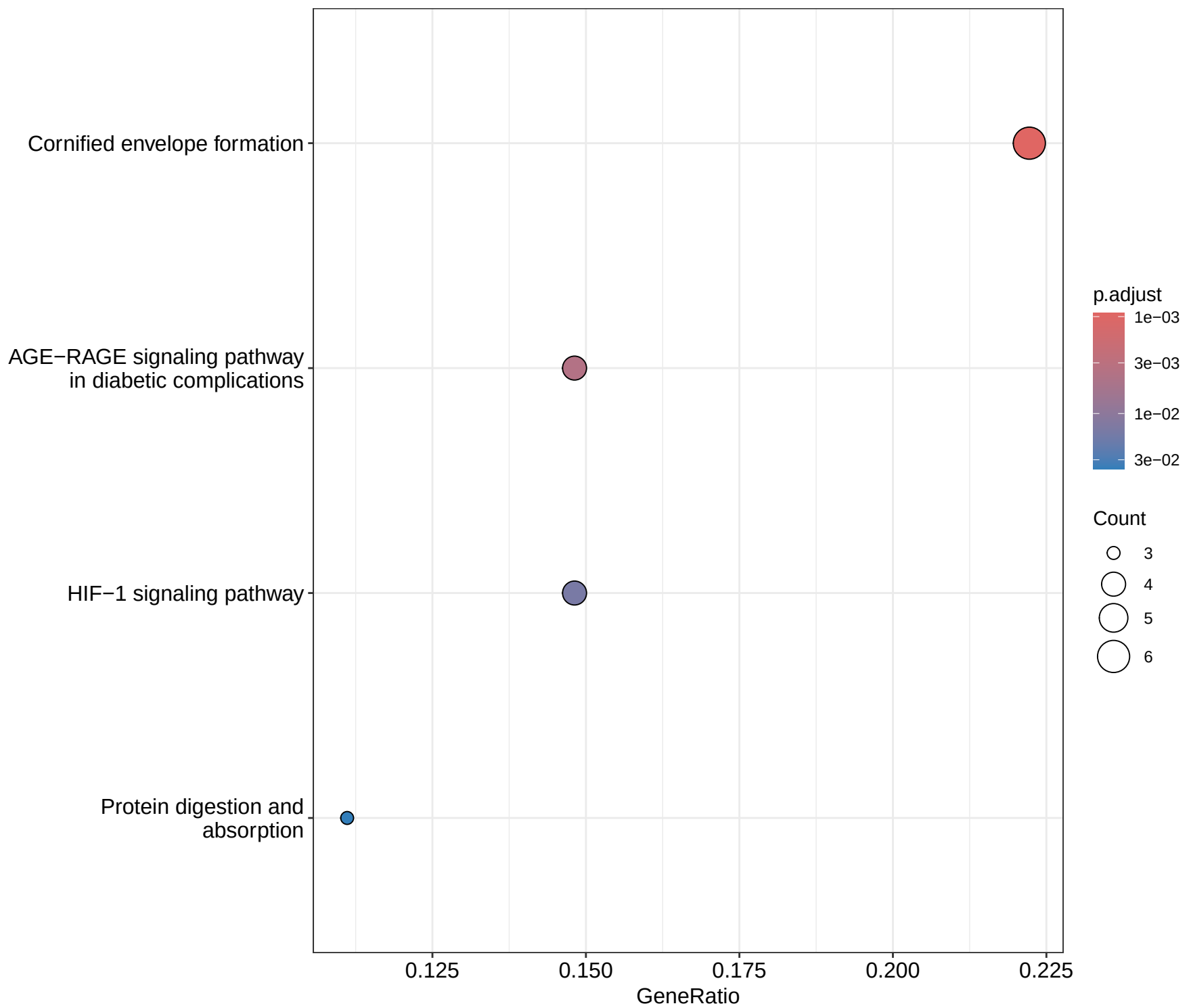
KEGG Pathways LPS_HI vs NaCl_HI
