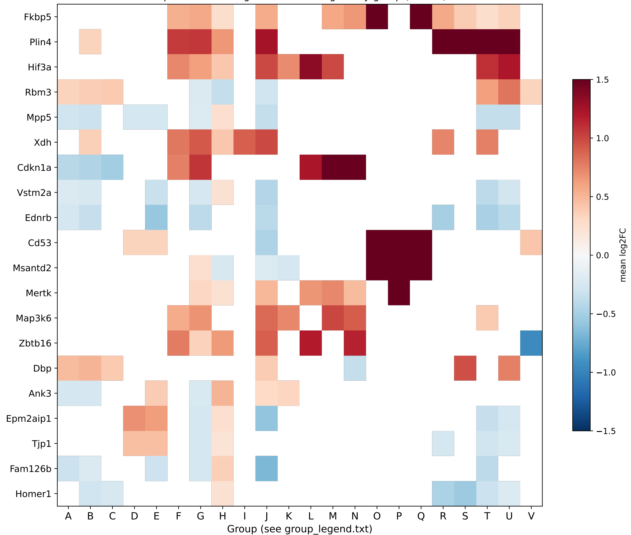
Top 20 consensus genes — mean log2FC by group (LFC0.2)
