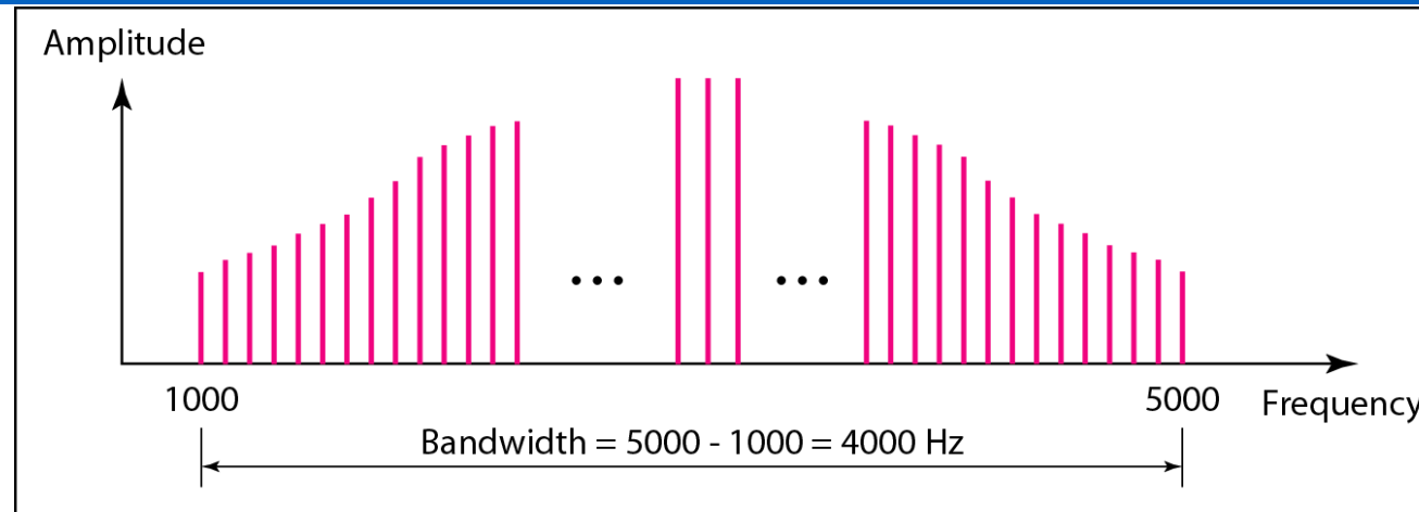
a. Bandwidth of a periodic signal
