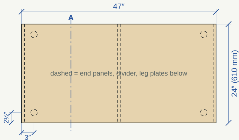
4 Top plan
