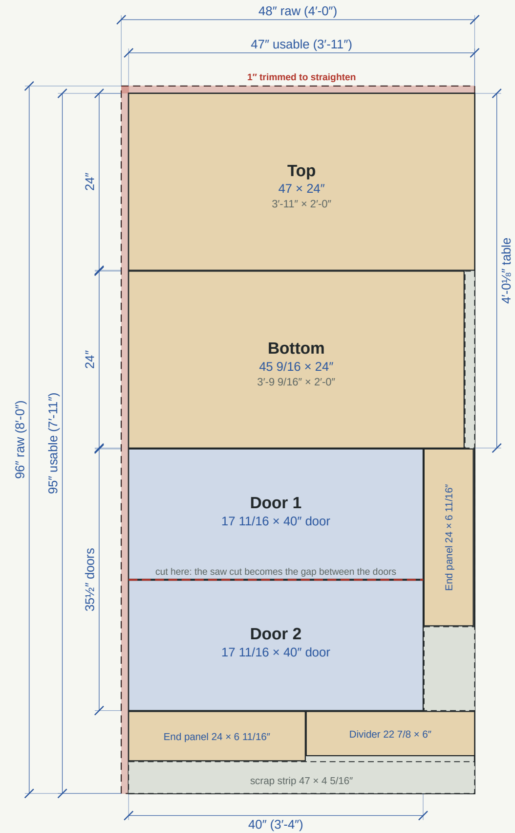
6 Sheet 1, stood upright: table + doors
