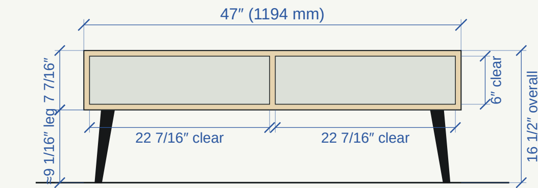
3 Front elevation
