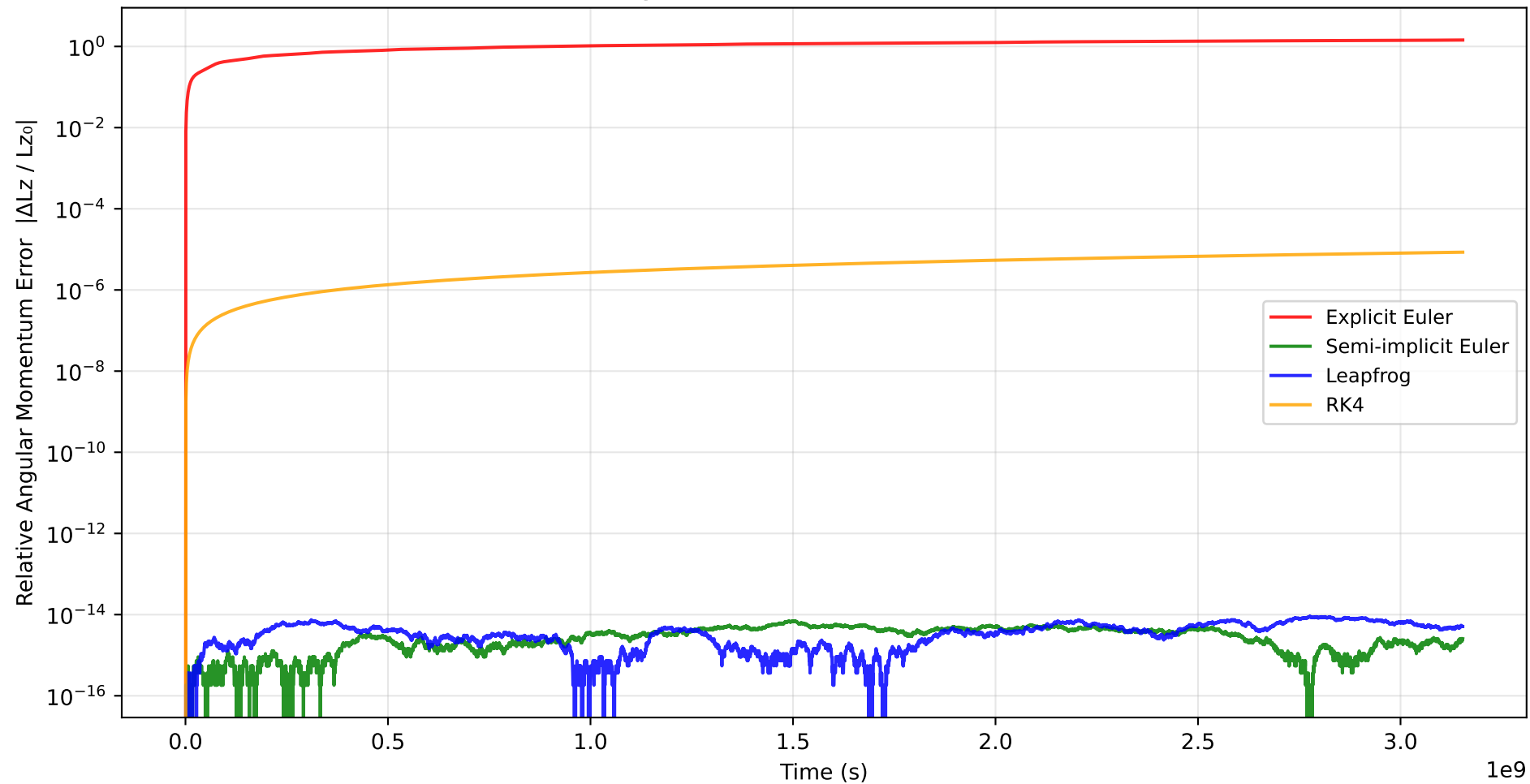
Total Angular Momentum Conservation Error
