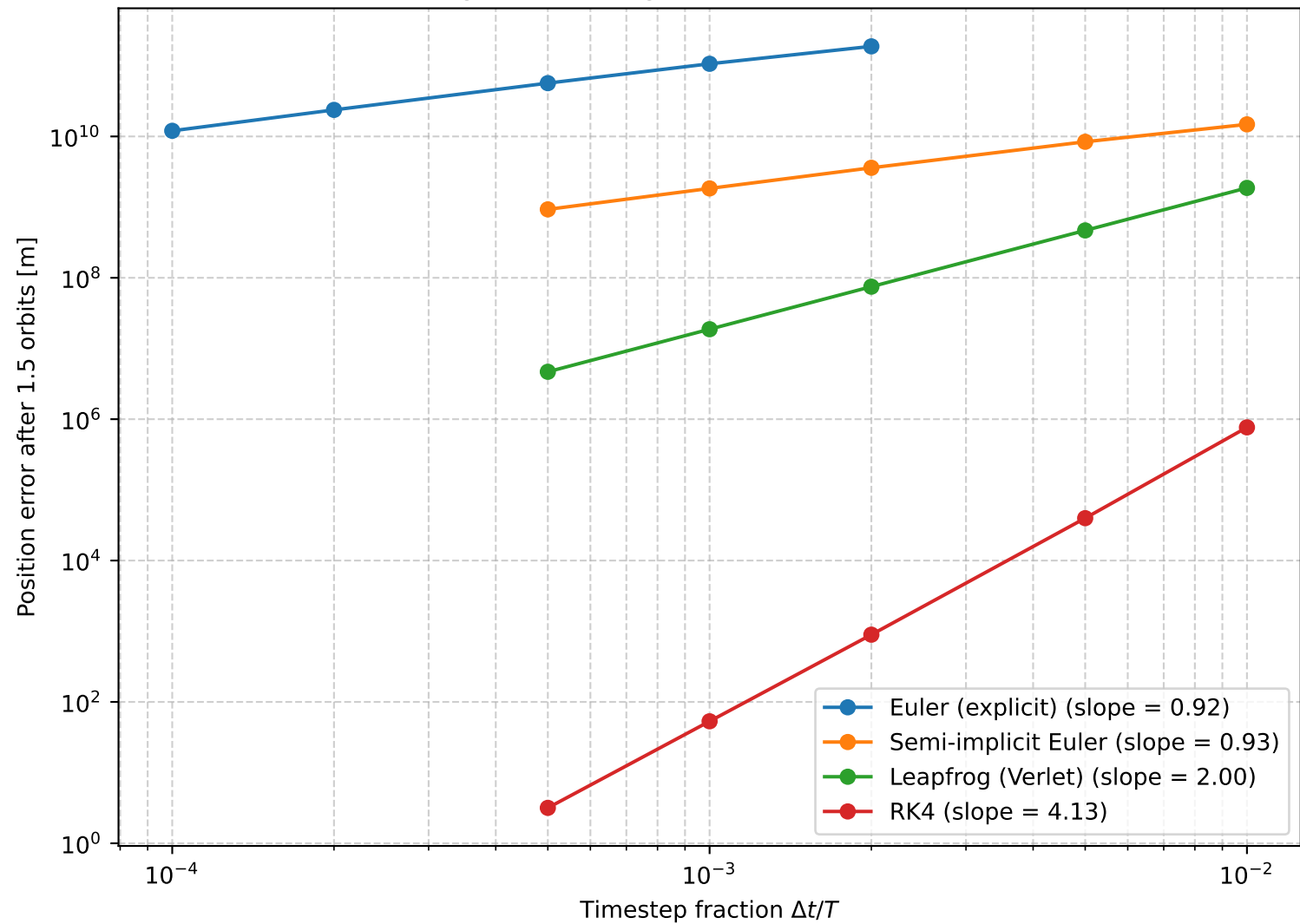
Convergence of integrators (Earth-Sun, 1.5 orbits)
