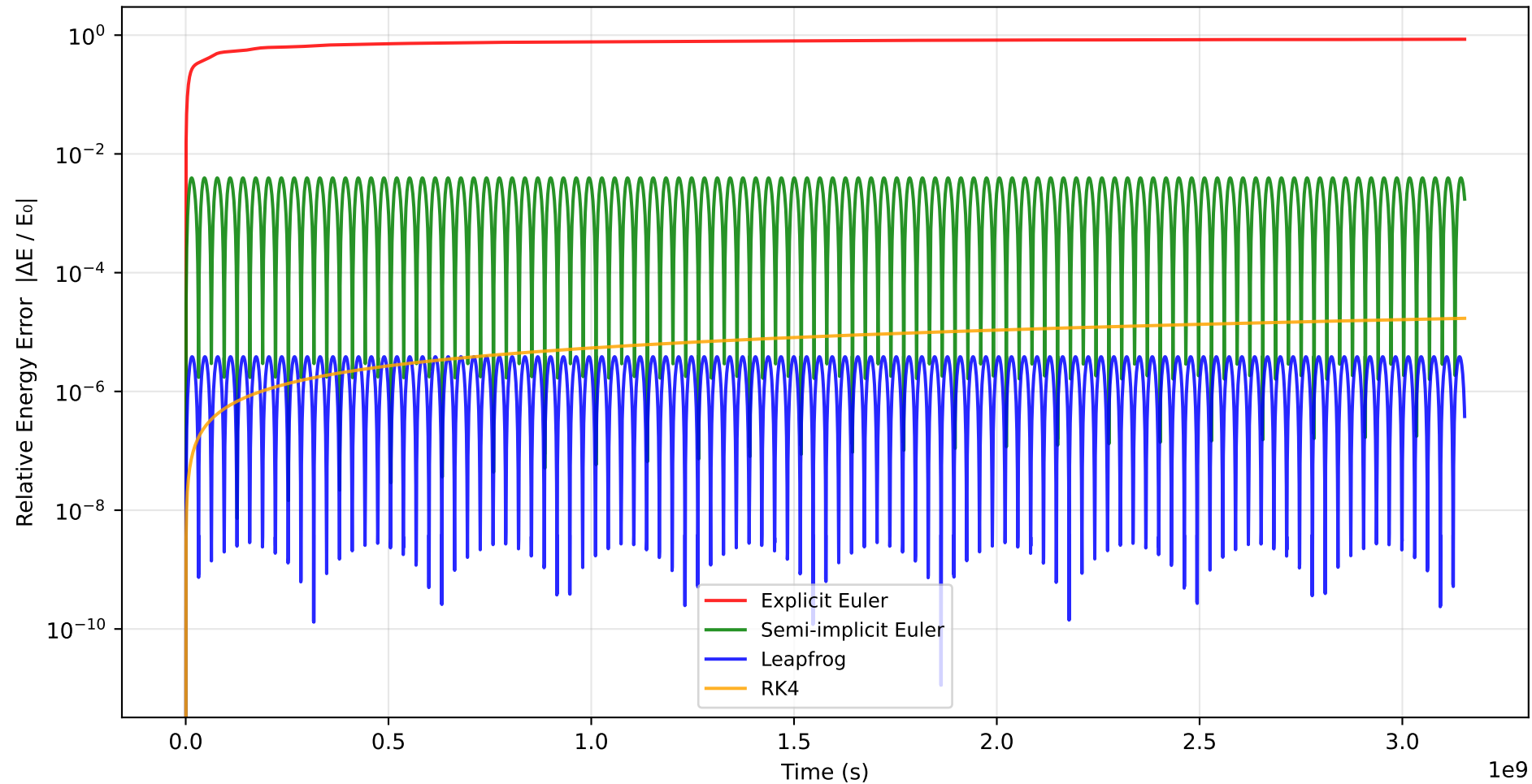
Total Energy Conservation Error
