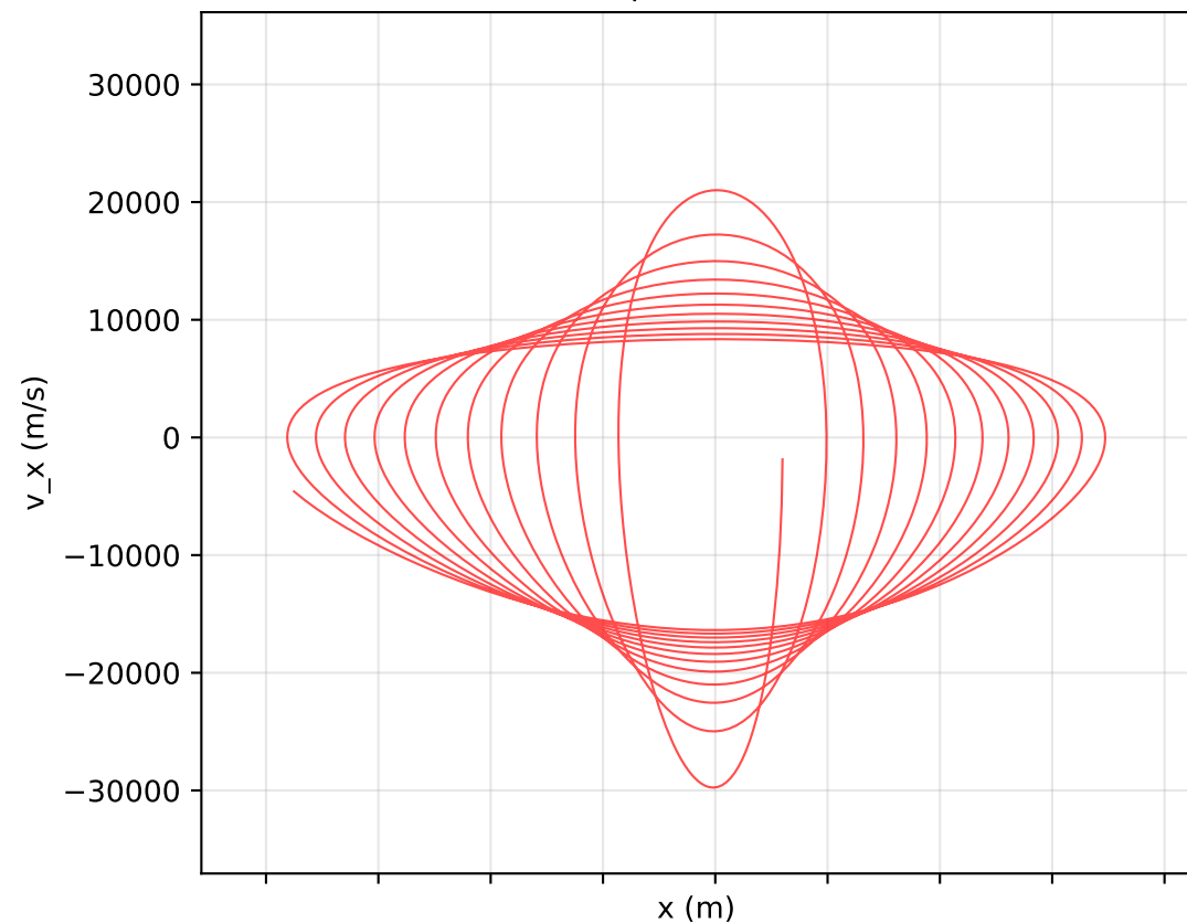
Leapfrog
