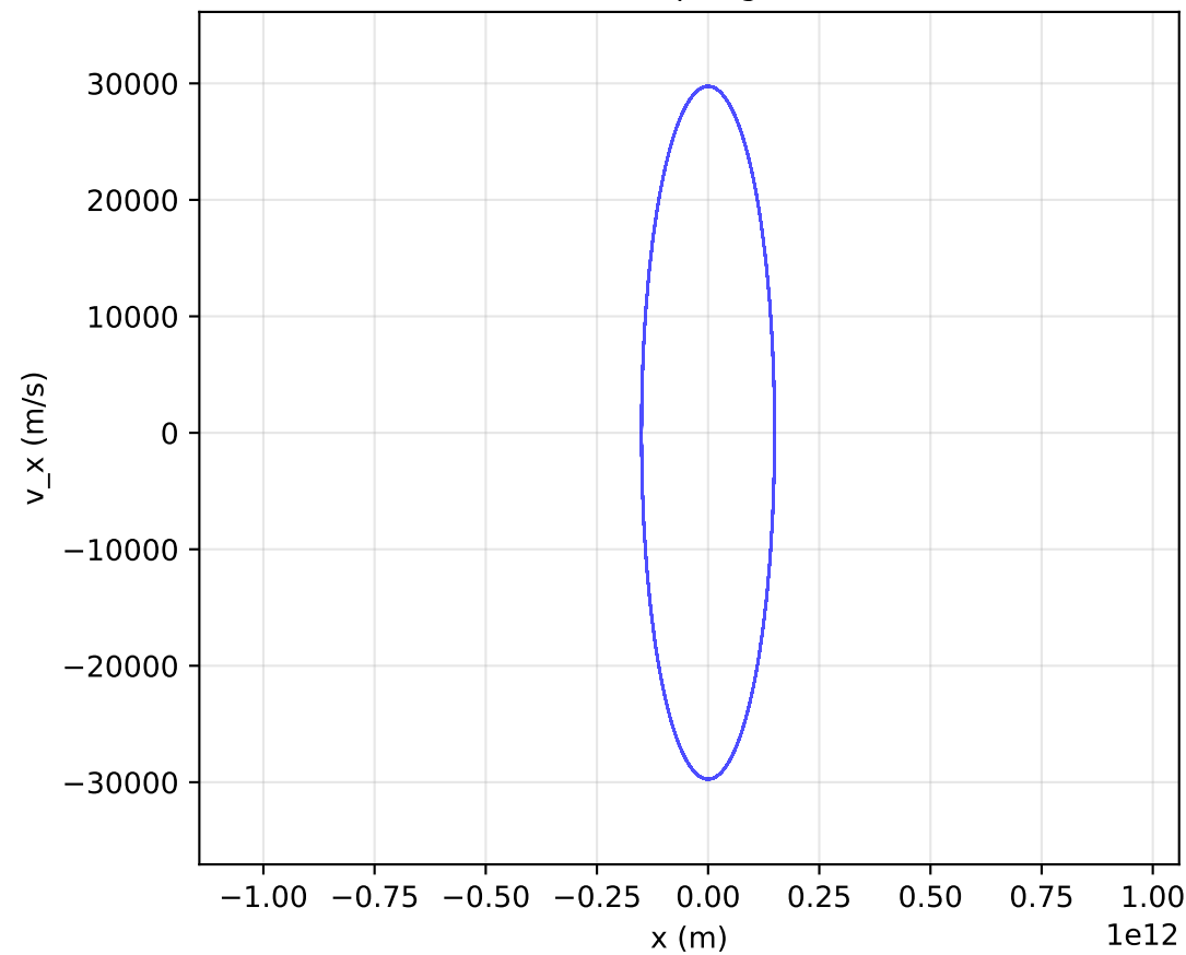
Leapfrog
