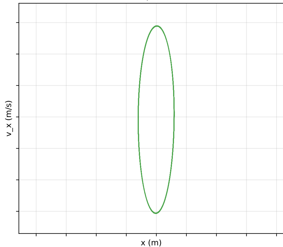
RK4
