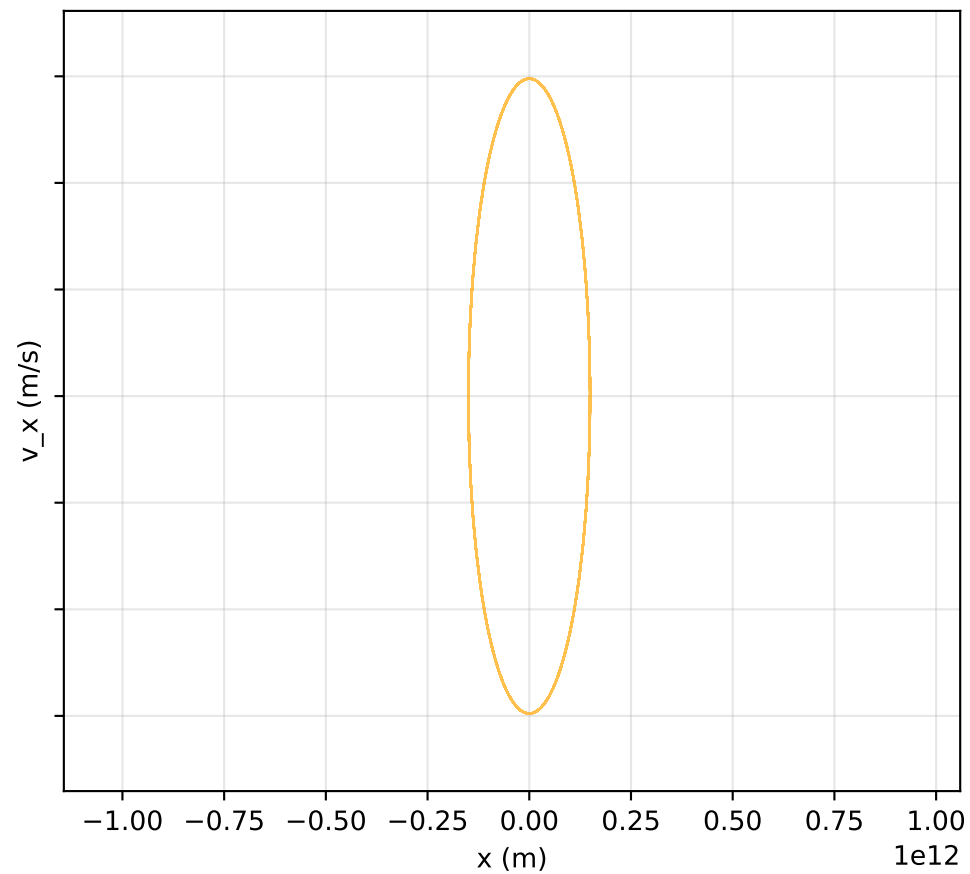
RK4
