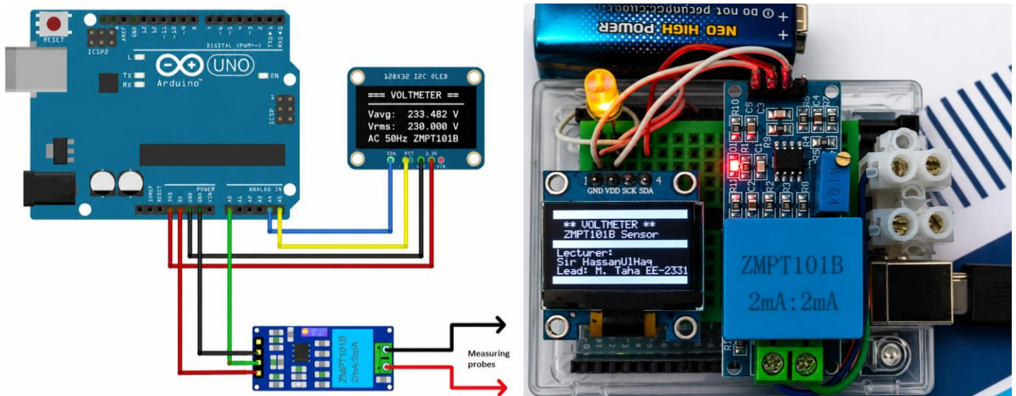
Figure 1: Hardware Setup – Arduino UNO with ZMPT101B Module
