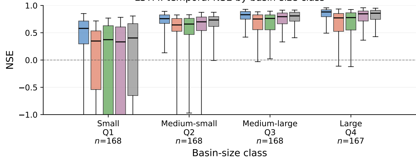
LSTM: temporal NSE by basin-size class
