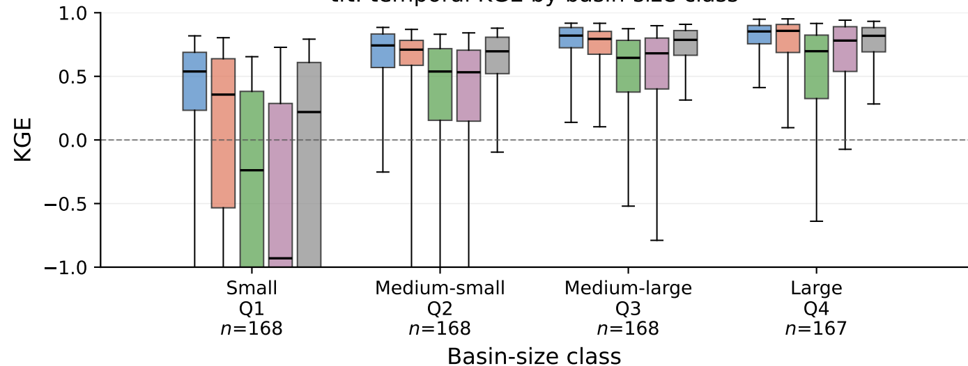
tit: temporal KGE by basin-size class
