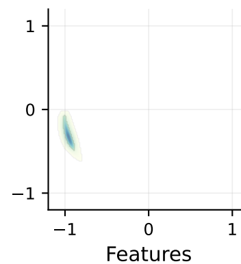
Cluster 0
