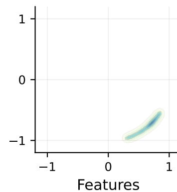
Cluster 3
