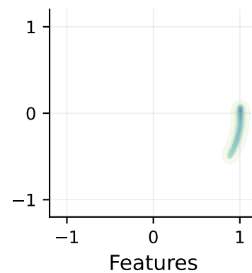
Cluster 4
