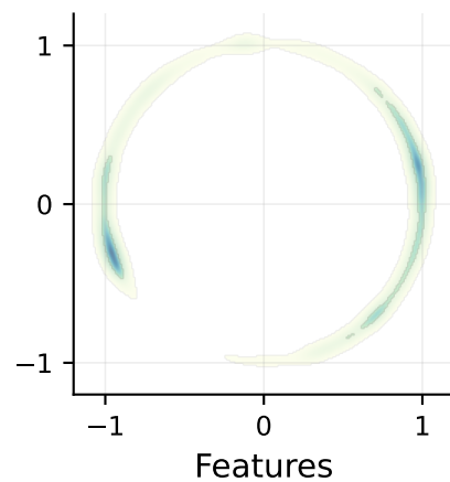
Feature Distribution
