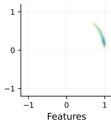
Cluster 1
