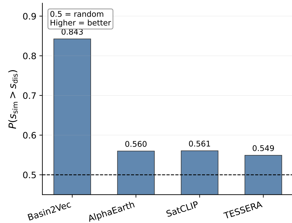
(c) Pair-ranking
