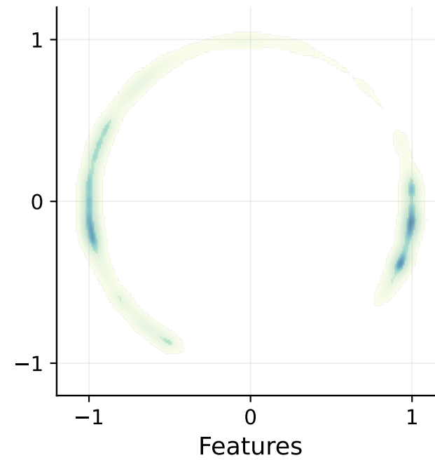
SatCLIP
