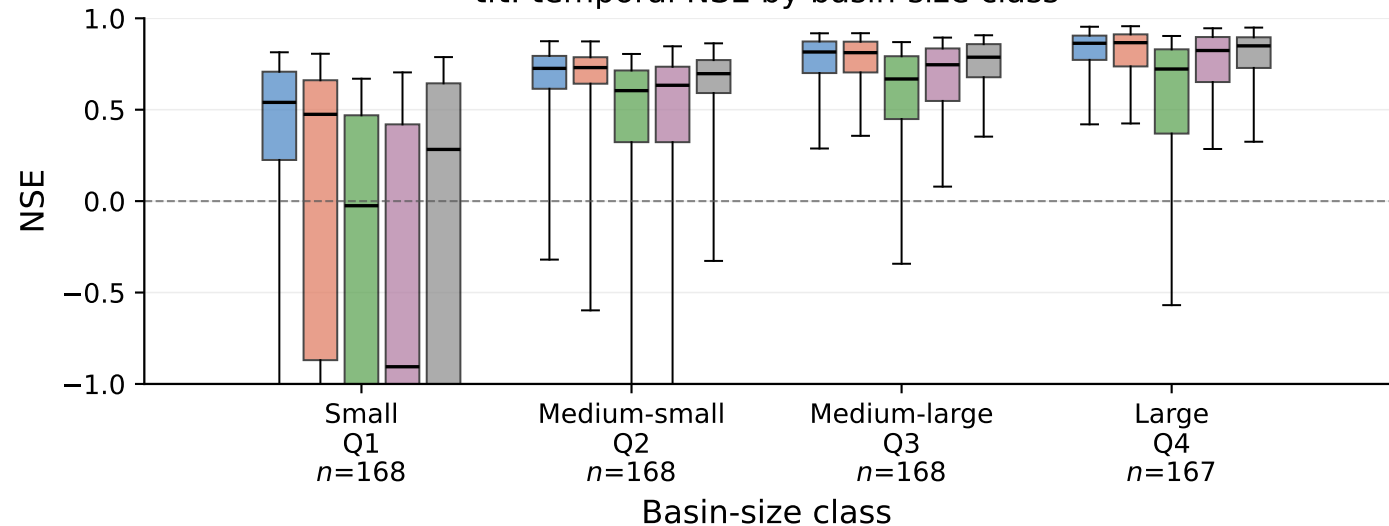
tit: temporal NSE by basin-size class
