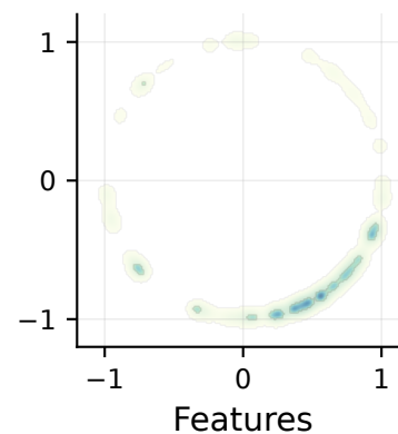
Cluster 5
