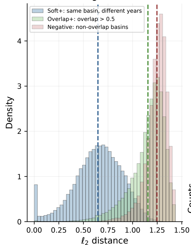
Positive and Negative Pair Distances
