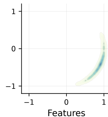
Cluster 3
