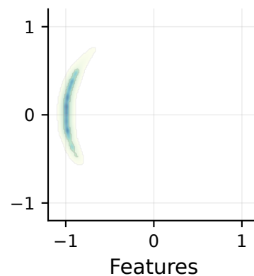
Cluster 6
