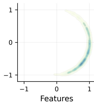
Cluster 2
