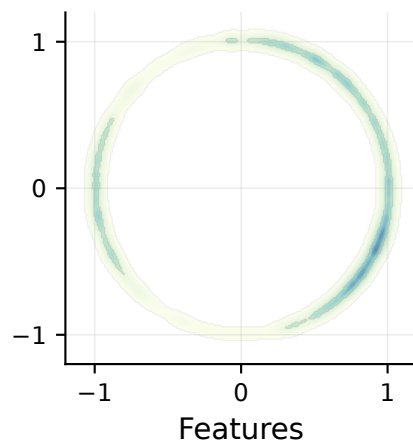
Feature Distribution
