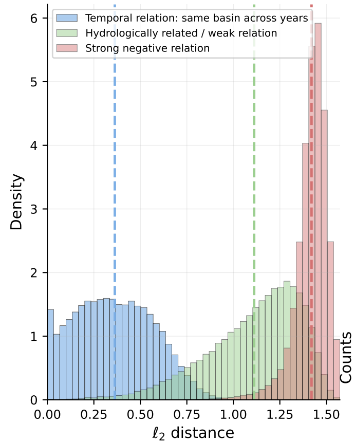
Grouped Relation-aware Pair Distances
