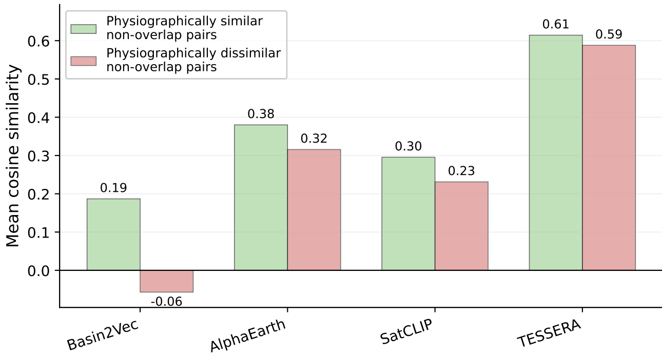
(a) Mean similarity
