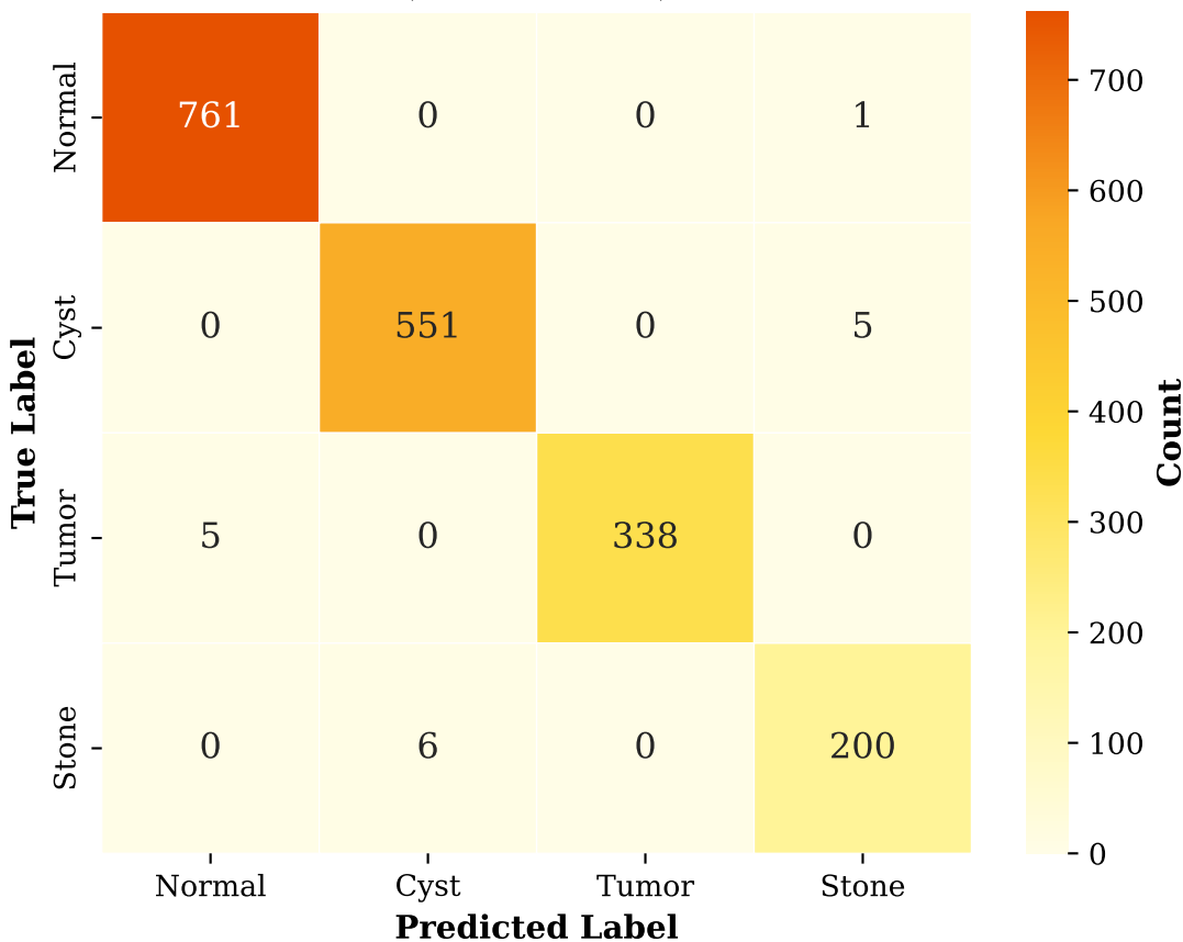
MUL-CNN -- Confusion Matrix (CT-KIDNEY)
