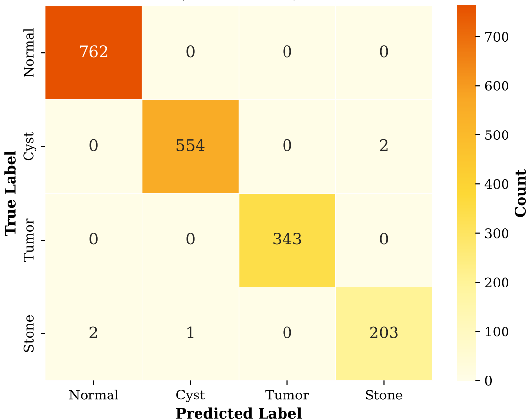
ResNet-50 -- Confusion Matrix (CT-KIDNEY)
