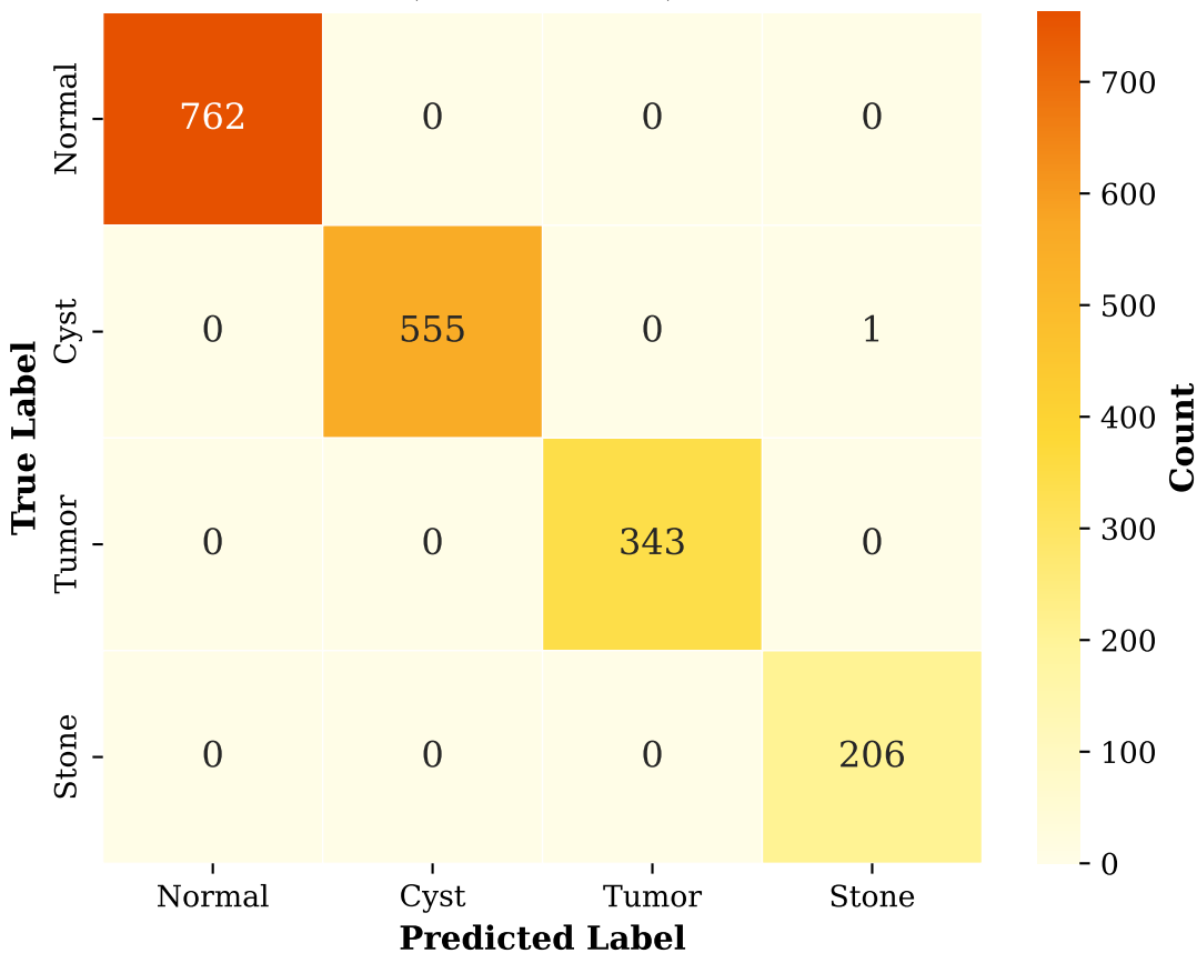
VGG-16 -- Confusion Matrix (CT-KIDNEY)
