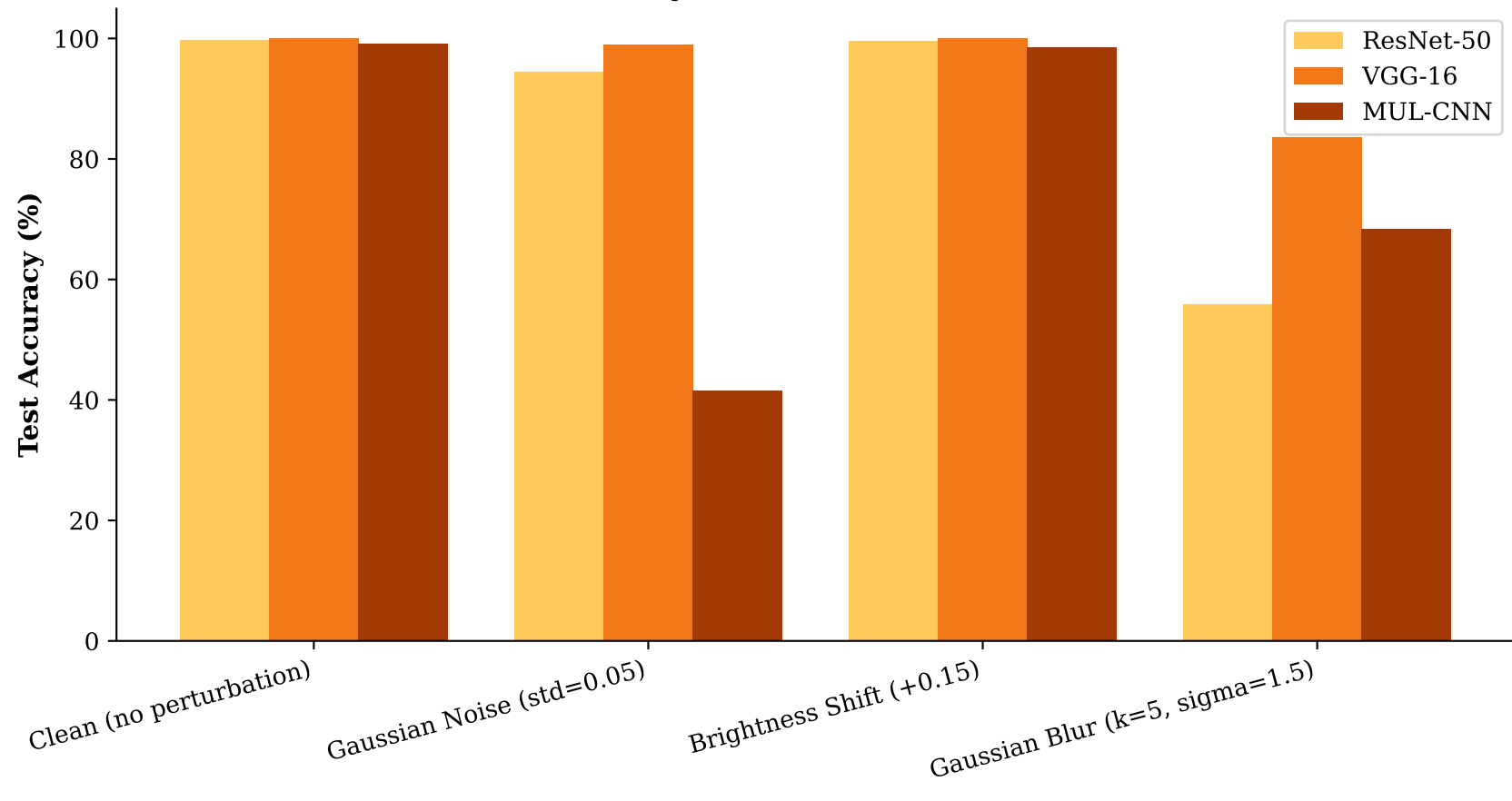
CT-KIDNEY: Accuracy Under Inference-Time Perturbation
