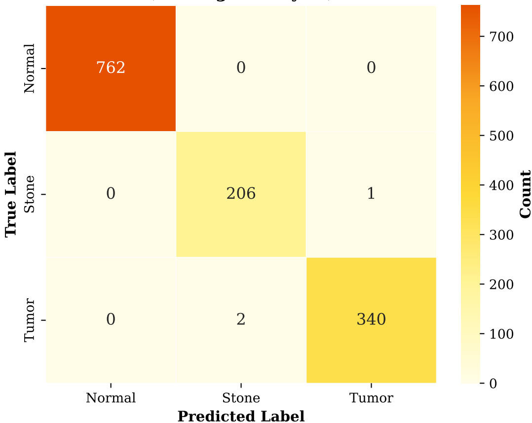
ResNet-50 -- Confusion Matrix (RenSeg-KidneyCT)
