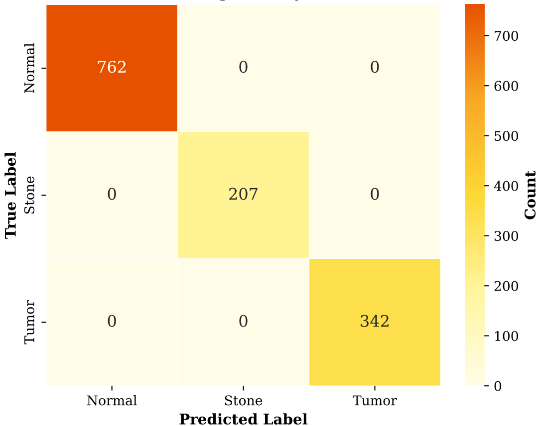
VGG-16 -- Confusion Matrix (RenSeg-KidneyCT)
