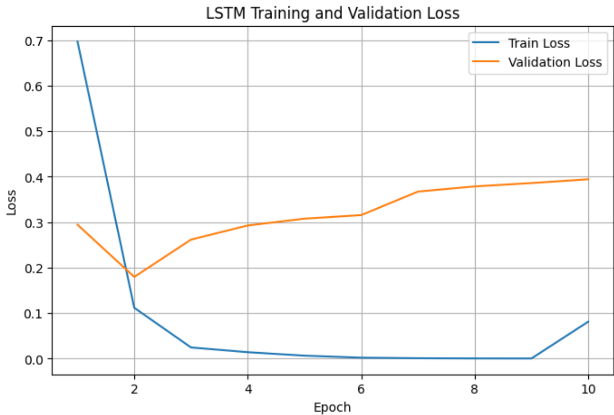
Figure 1. LSTM training and validation loss over 10 epochs.
