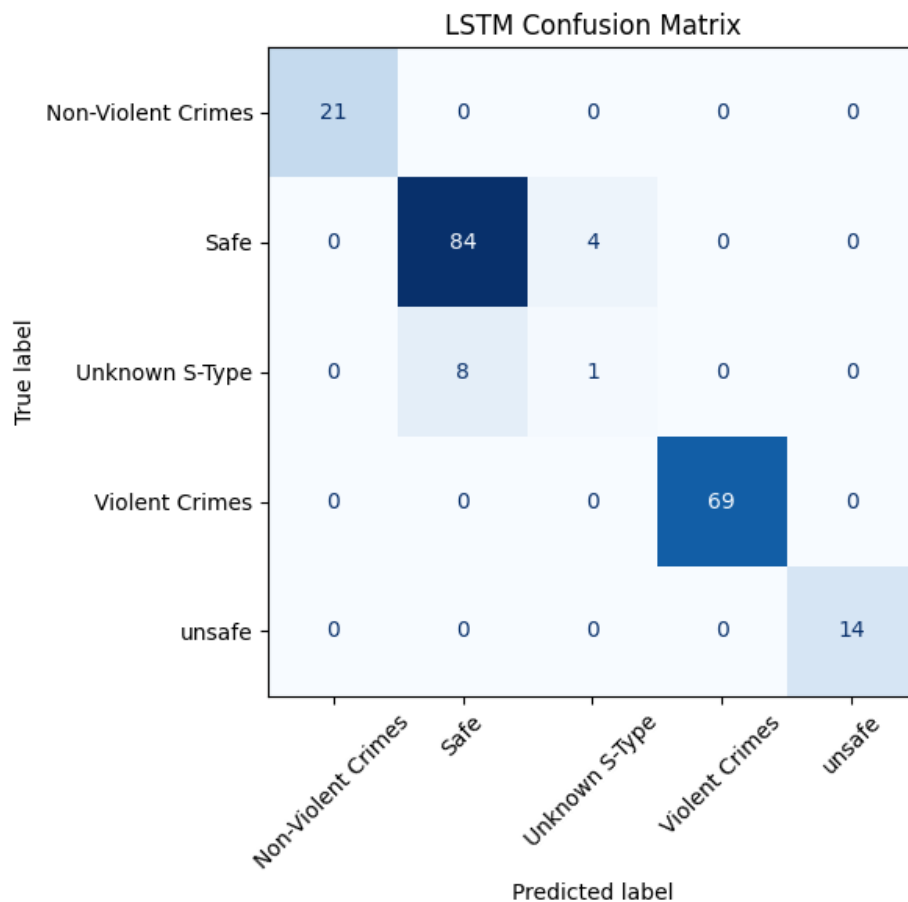
Figure 3. LSTM confusion matrix on the test set (201 examples).
