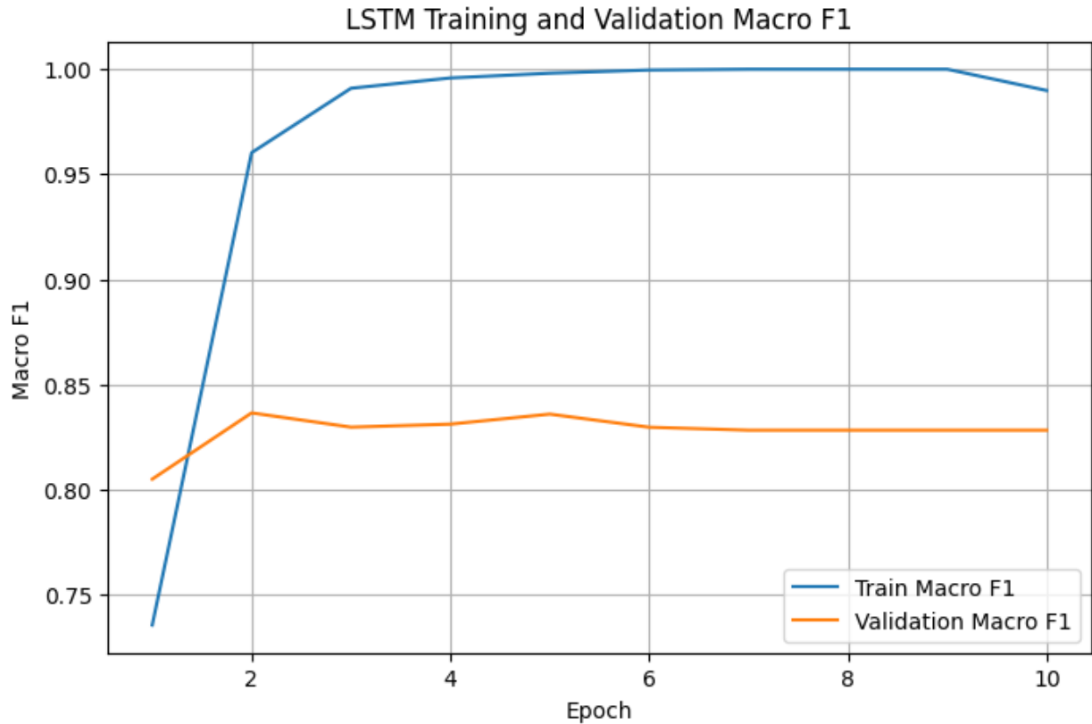
Figure 2. LSTM training and validation macro F1 over 10 epochs.
