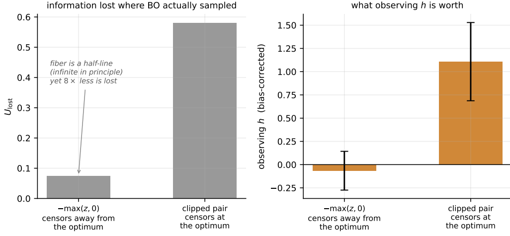
Figure 4: The finding. The map with the larger fiber loses less where BO looks, and observing h buys it nothing.
