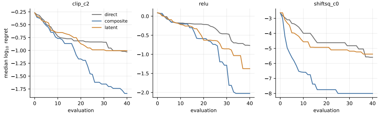
Figure 5: Median convergence over the pooled runs, uncorrected : each latent-composite gap still contains the +0.409 handicap measured on identity . On relu that handicap is most of the visible gap.
