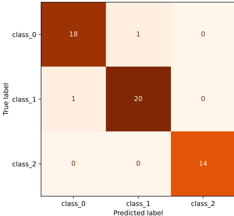
MultinomialNB — Confusion Matrix
