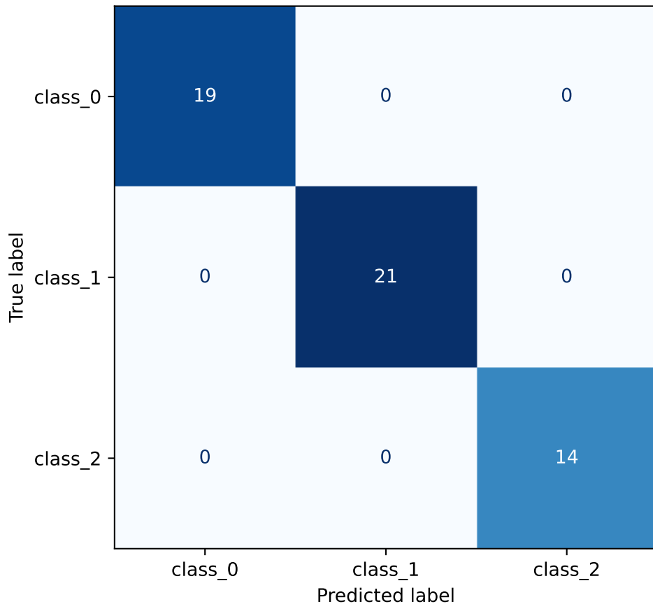
GaussianNB — Confusion Matrix
