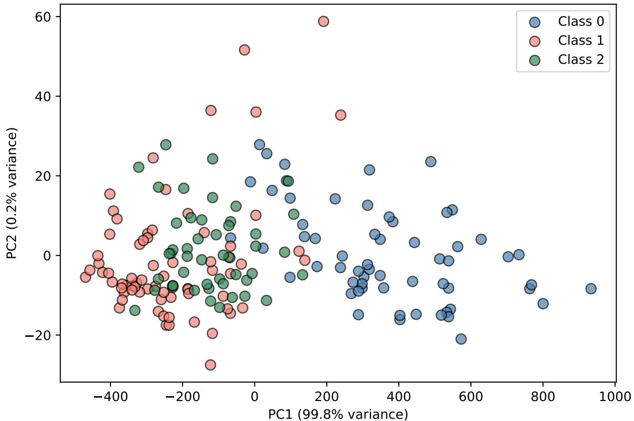
PCA 2D Projection of Wine Dataset
