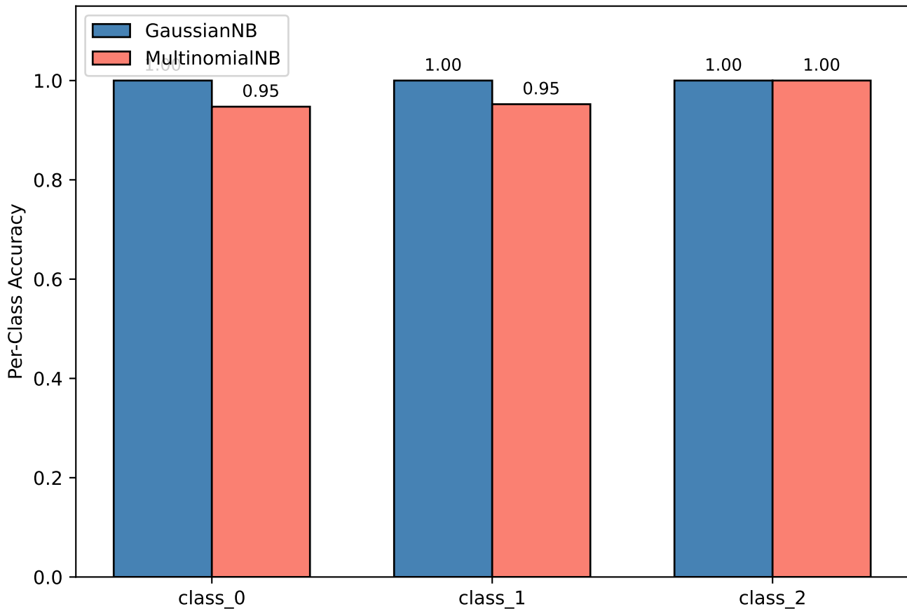
Per-Class Accuracy: GaussianNB vs MultinomialNB
