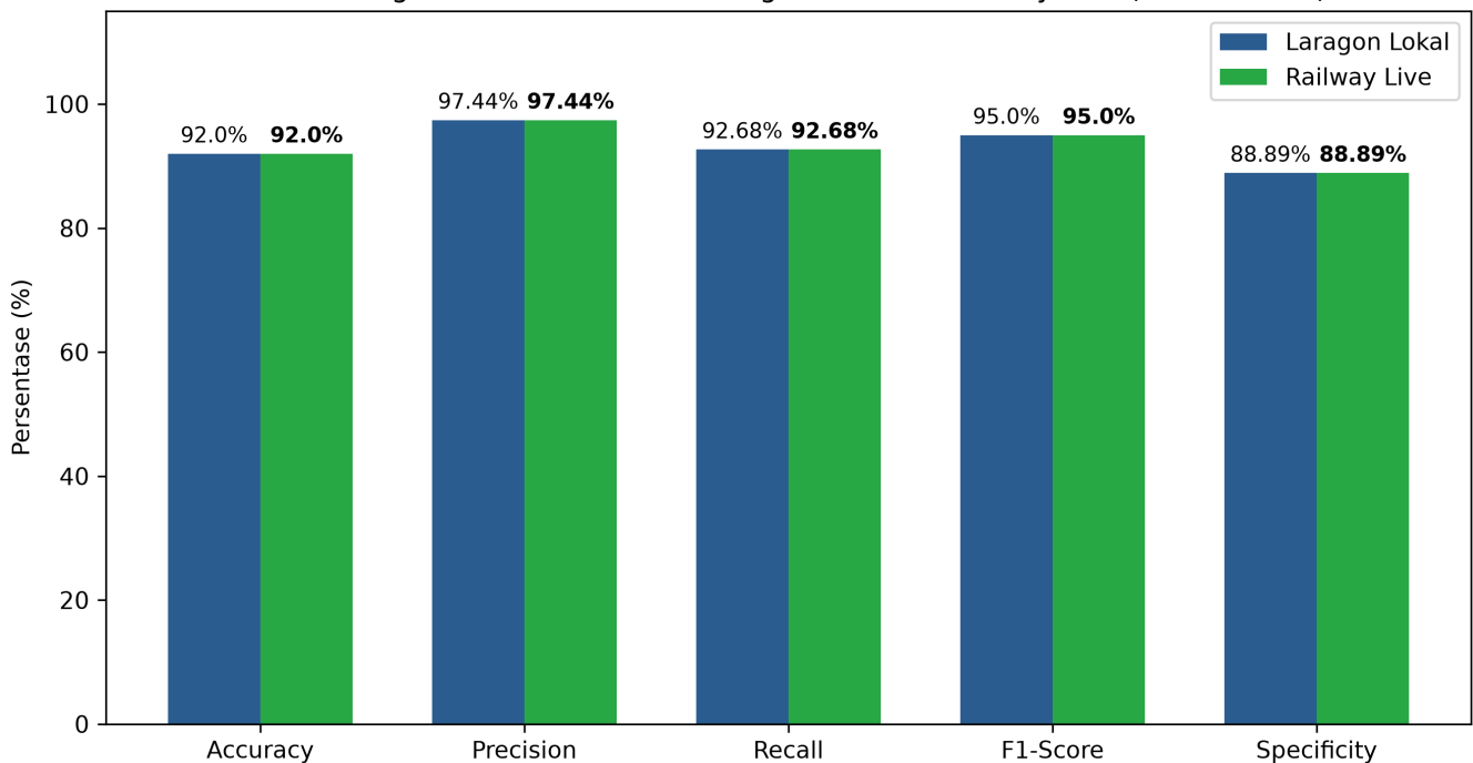
Perbandingan Metrik Performa: Laragon Lokal vs Railway Live (100 Gambar)
