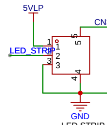
LED STRIP
