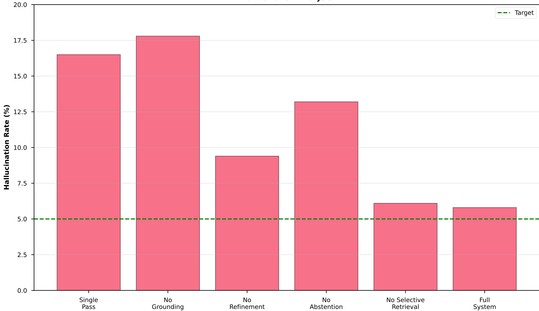
Hallucination Analysis
