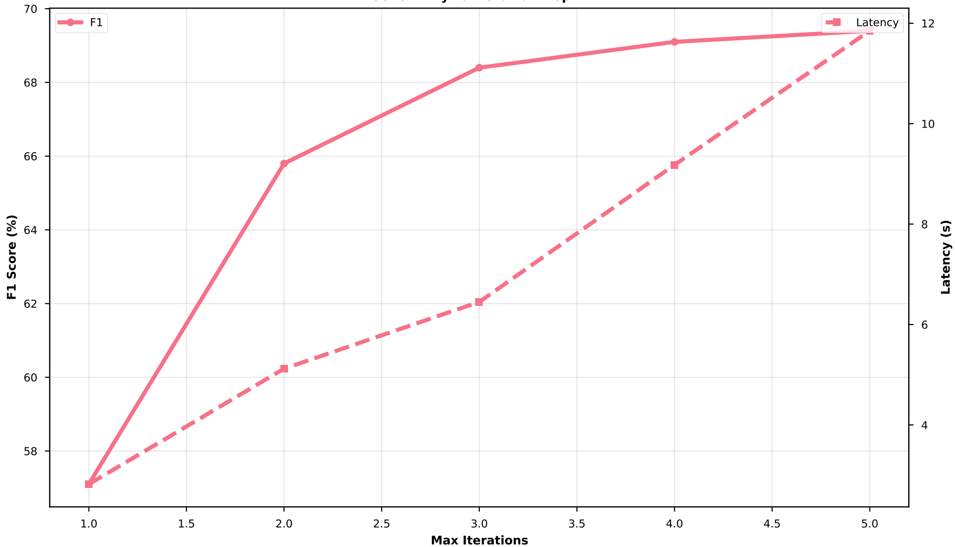
Sensitivity to Iteration Depth
