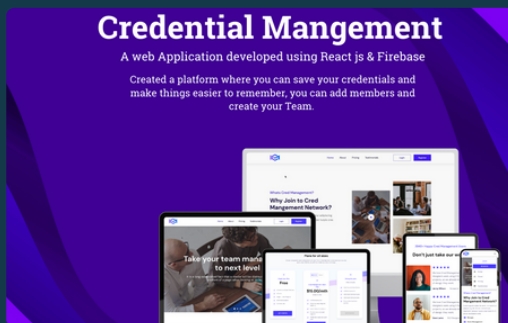
Credential Management
